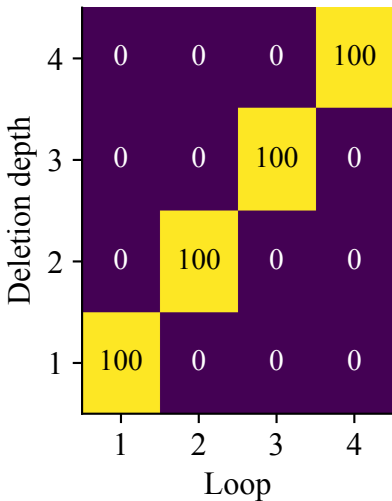
(a) Stepwise
