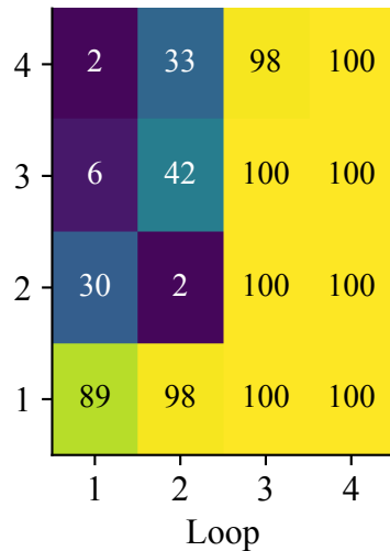
(b) Final-only
