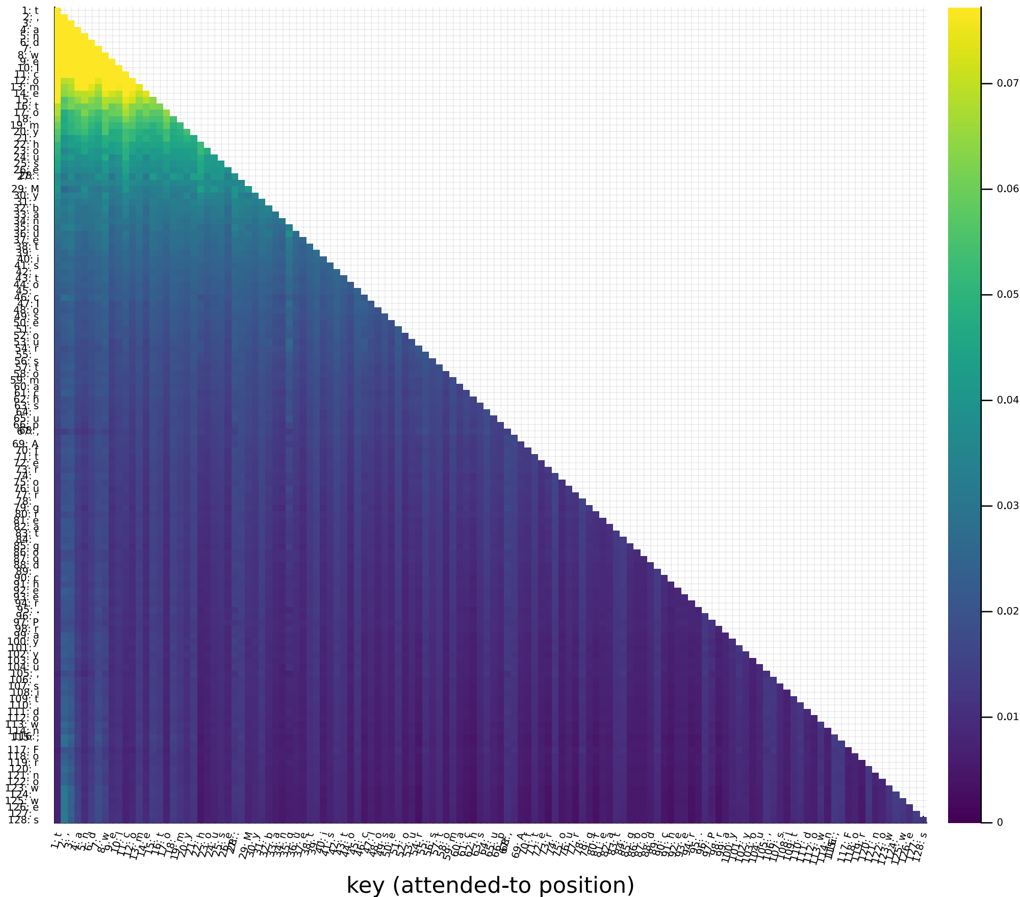
Causal attention weights, layer 1, head 1
