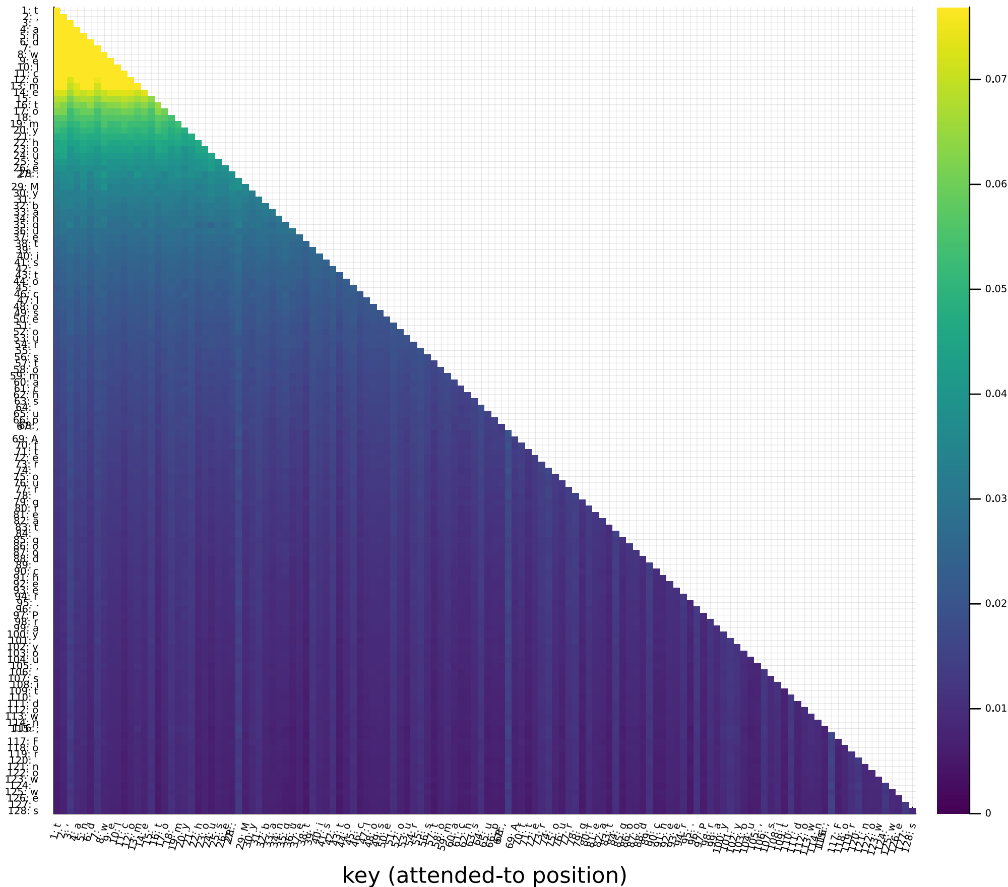
Causal attention weights, layer 1, head 4
