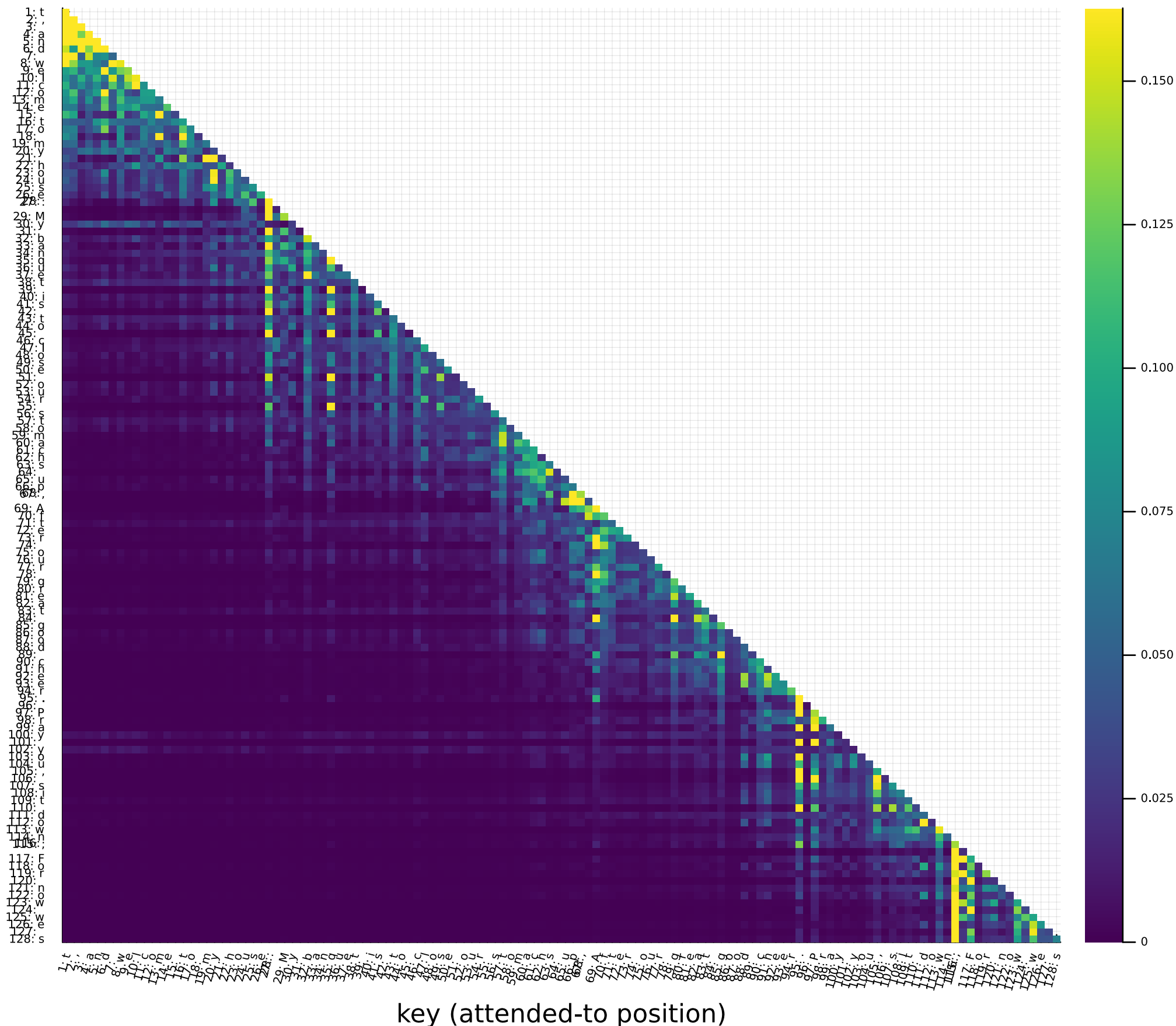
Causal attention weights, layer 1, head 8
