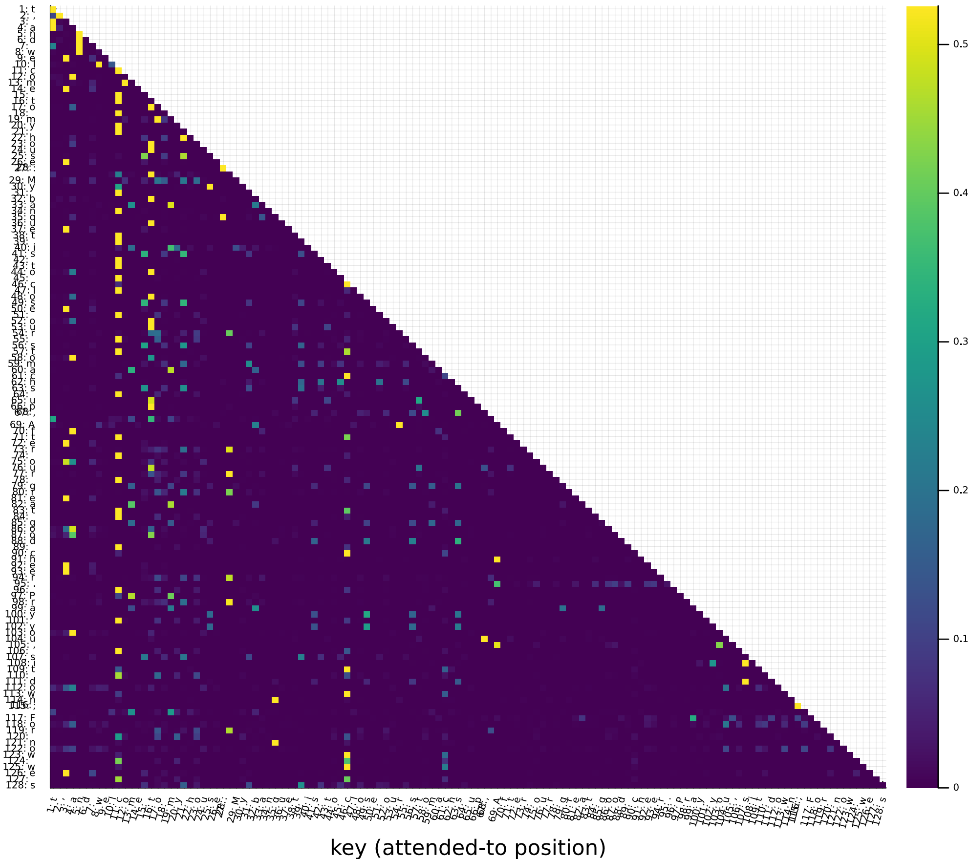
Causal attention weights, layer 4, head 1
