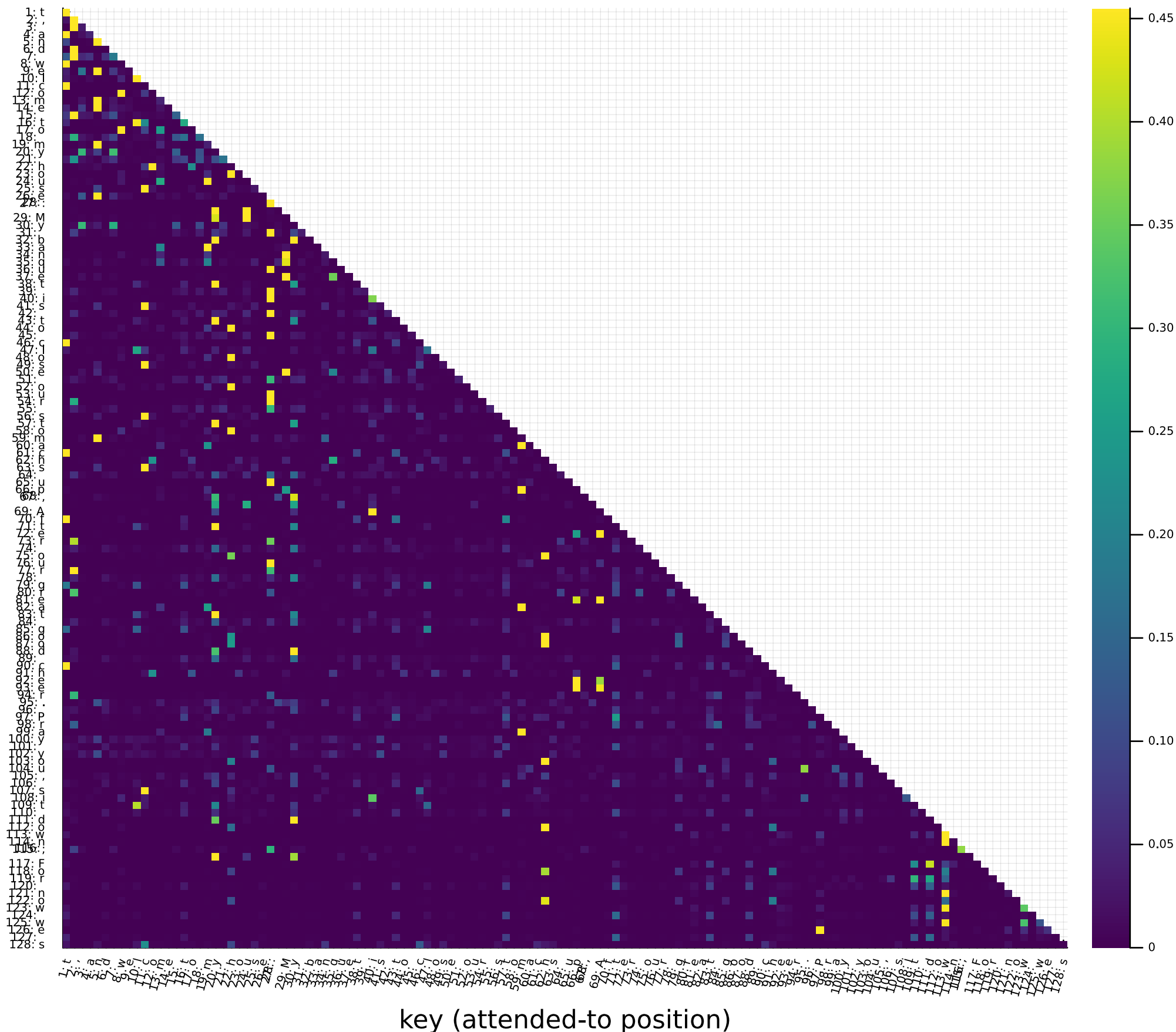
Causal attention weights, layer 4, head 8
