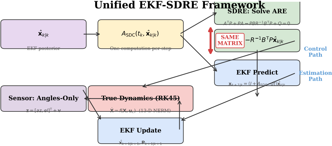
Fig. 2. Unified EKF-SDRE algorithm flow — single A_{SDC}(t_k) drives both control and estimation.
