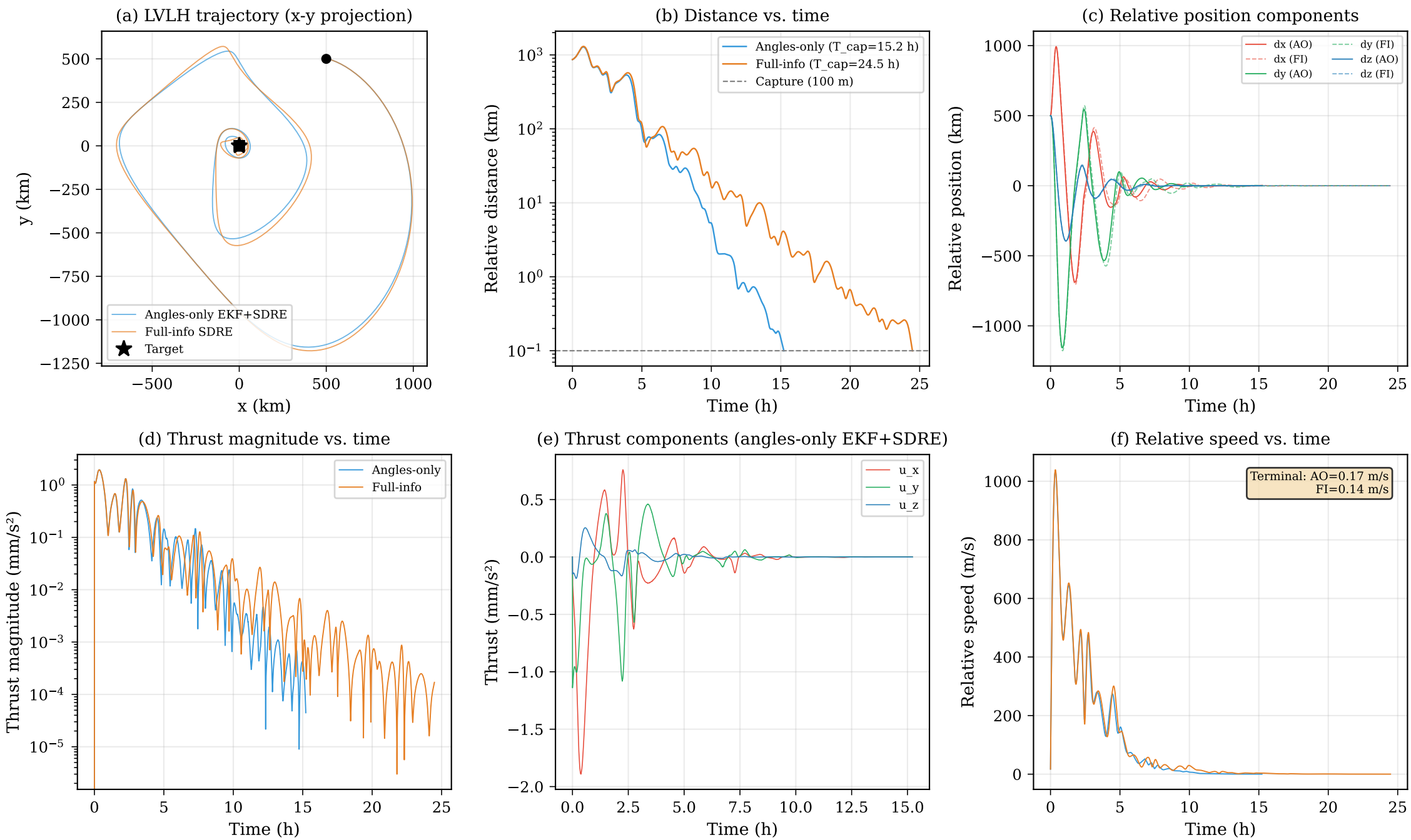
Fig. 4. Baseline comparison: angles-only EKF+SDRE vs. full-information SDRE.
