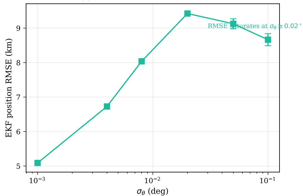
(c) Estimation error vs. sensor noise
