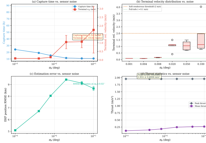
Figure 6: Sensor noise sensitivity analysis the speed-softness trade-off. (a) Capture time and terminal relative velocity versus \sigma_\theta (dual y-axis): a 100× noise increase reduces approach time by a factor of 2.3 but increases terminal v_{rel} by a factor of ~20 (0.09 m/s → 1.76 m/s). The dotted reference lines mark full-information SDRE baselines. (b) Terminal v_{rel} boxplot across seeds per noise level, with the 2 m/s soft-rendezvous safety threshold and full-information reference. Variance grows substantially above \sigma_\theta = 0.01^\circ . (c) EKF position RMSE versus \sigma_\theta , showing estimation error saturation above \sim 0.02^\circ . (d) Thrust mean and peak versus \sigma_\theta : peak thrust remains constant at \sim 1.96 m/s 2 , while mean thrust increases monotonically with noise.
