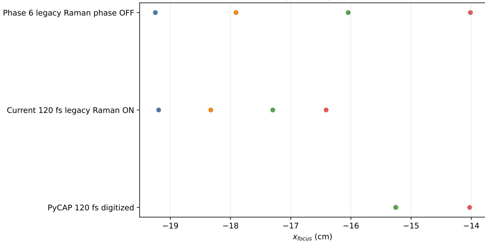
First density crossings (unshifted)
