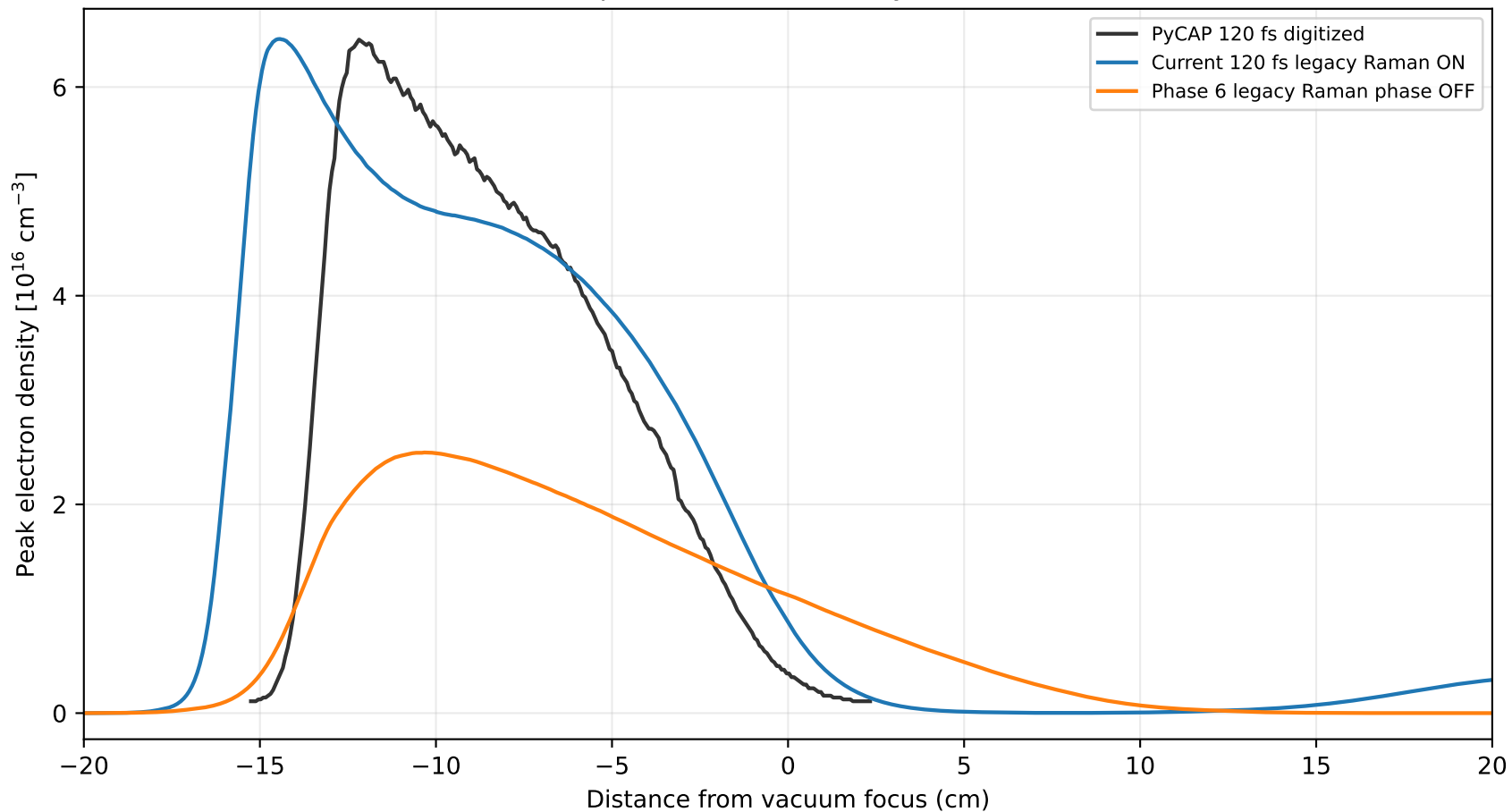
120 fs peak electron density (unshifted)
