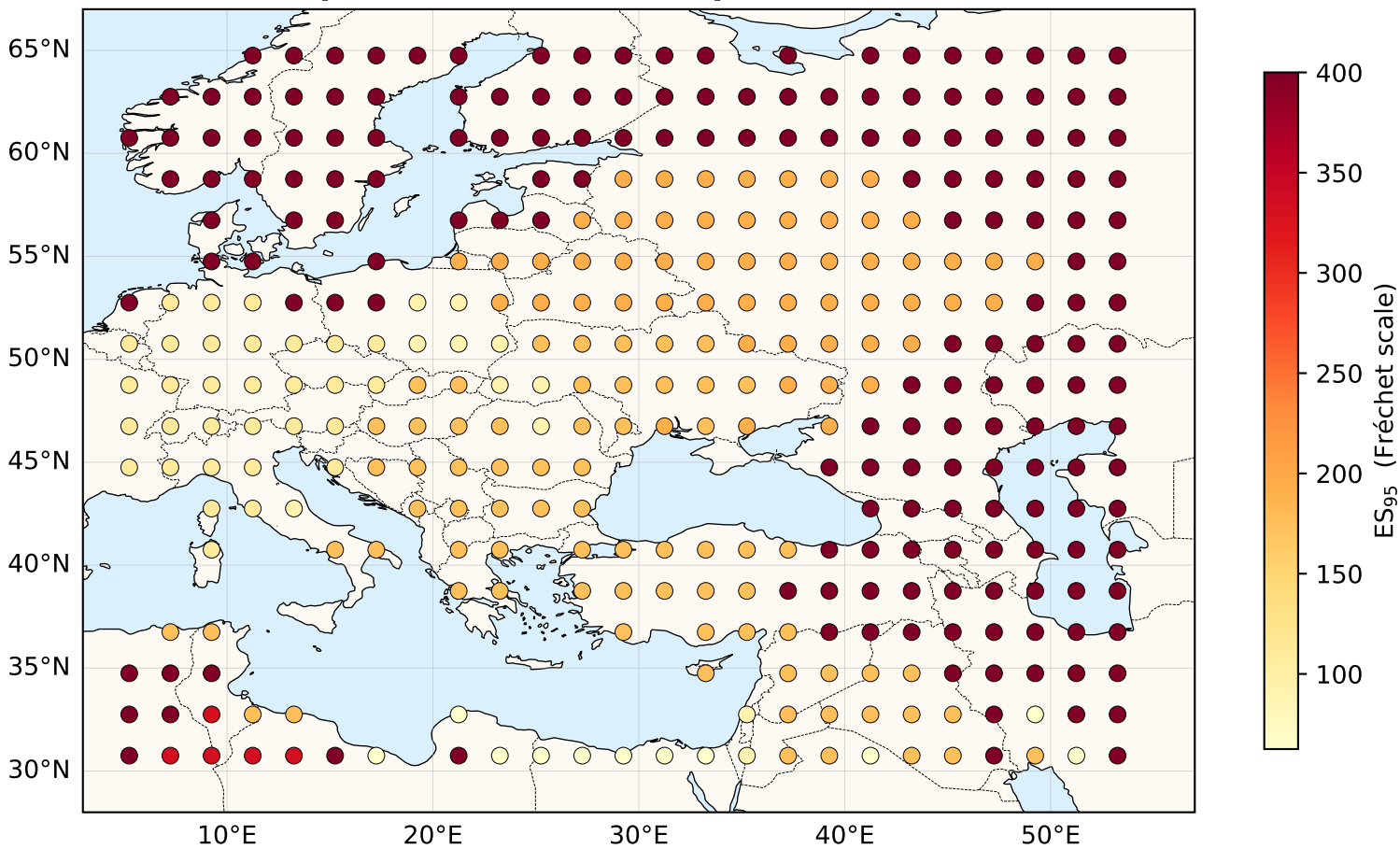
Expected Shortfall ES_{95} per EDC Cluster
