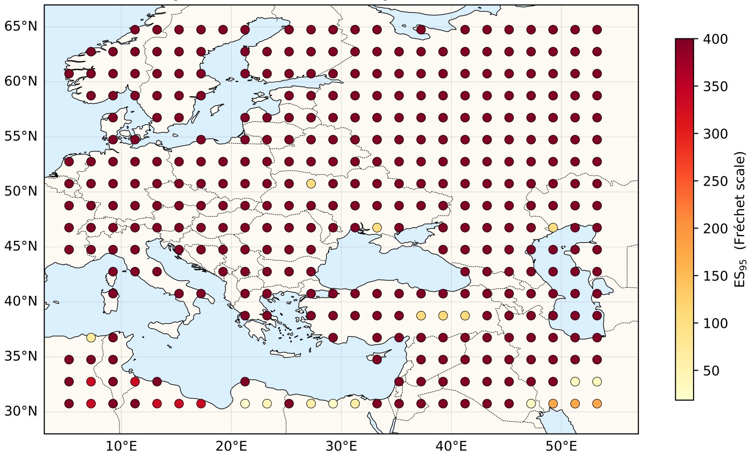
Expected Shortfall ES_{95} per LEC Cluster
