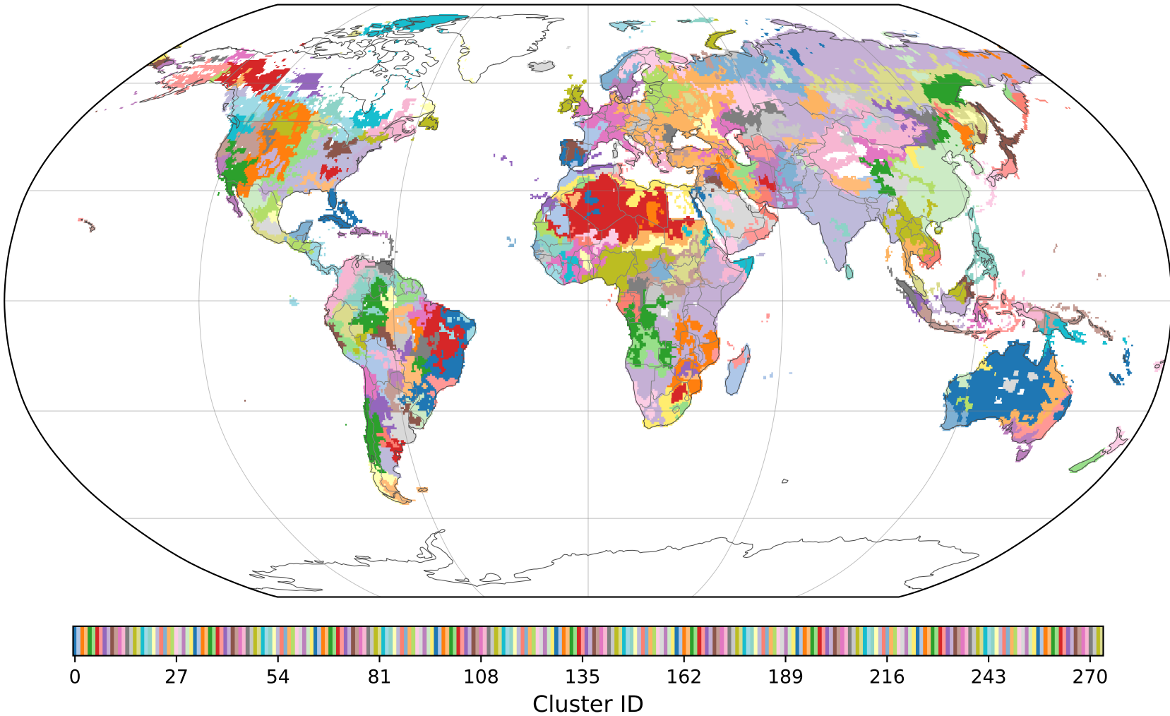
ES 95 Risk Clusters (274 regions)
