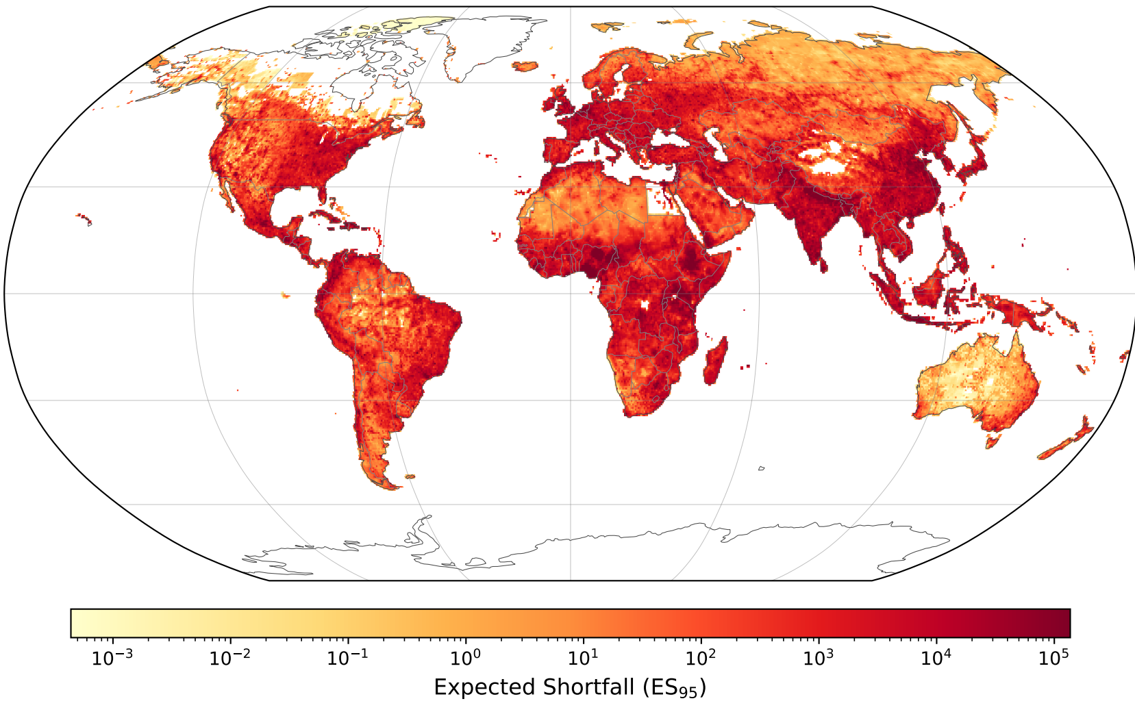
Global Expected Shortfall (95 %)
