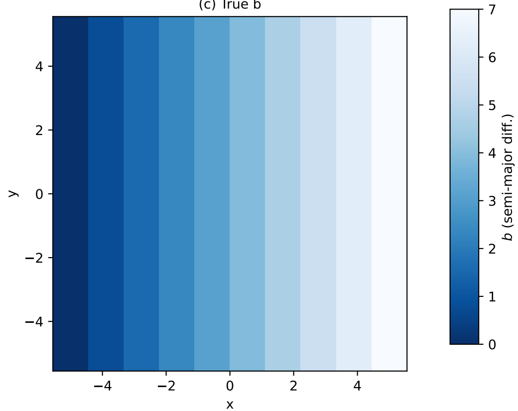
(c) True b
