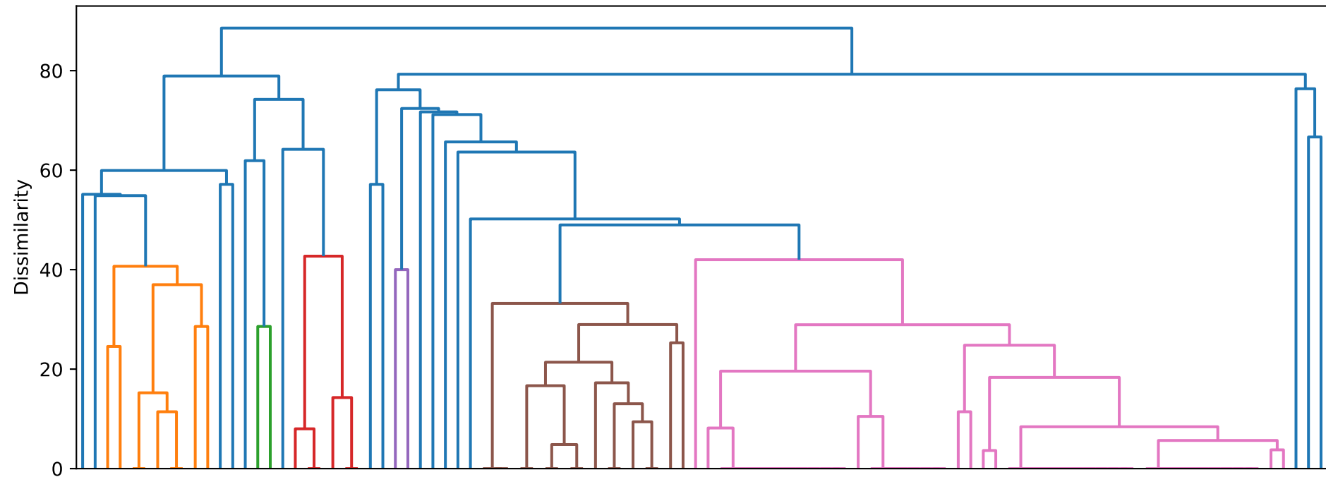
LEC dendrogram — stripes
