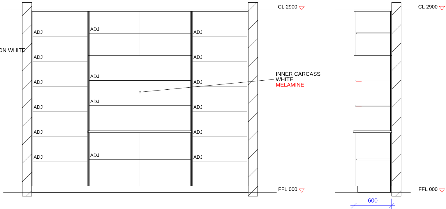
SECTION X-X 1:35
