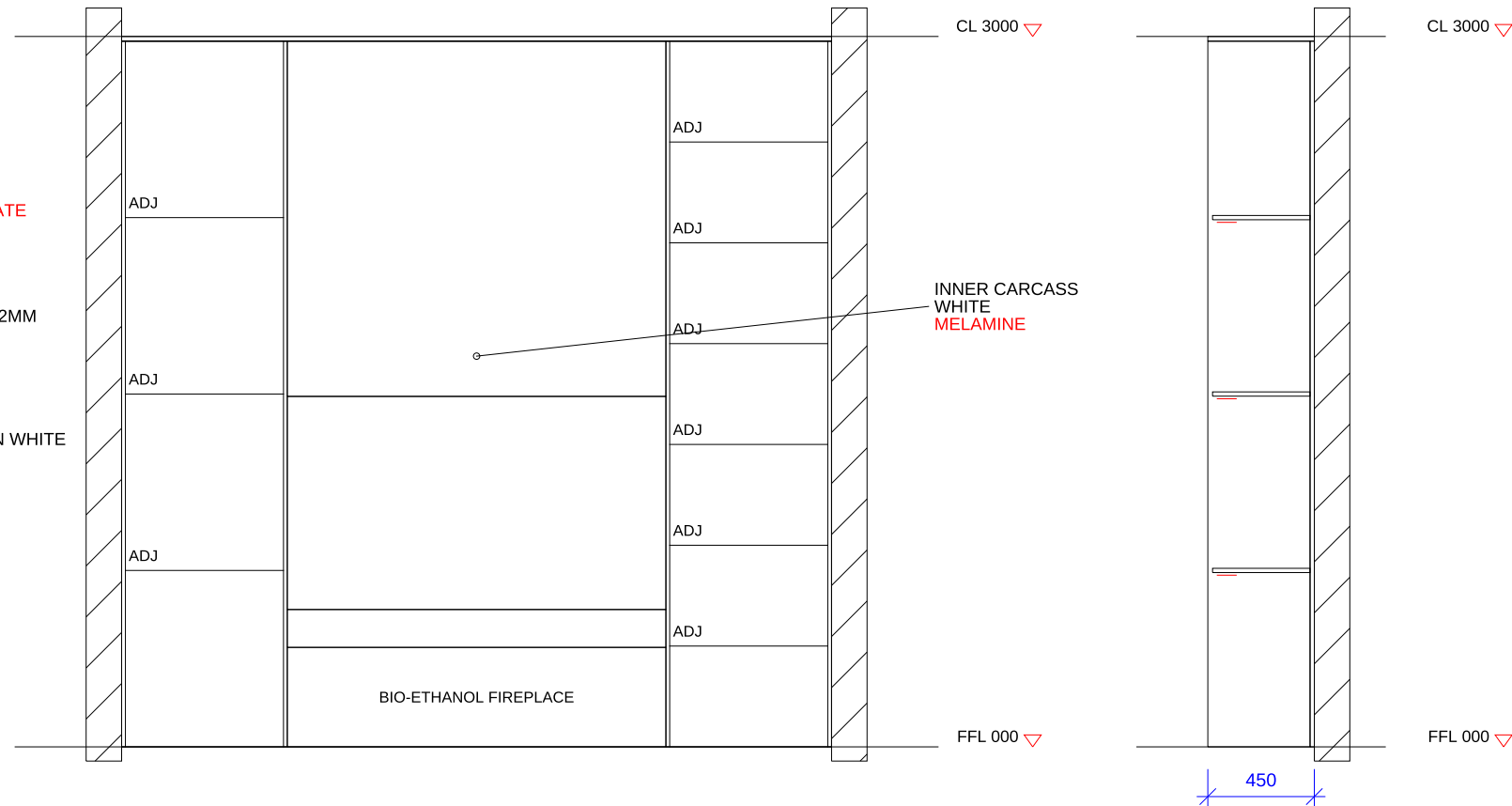
SECTION X-X 1:30
