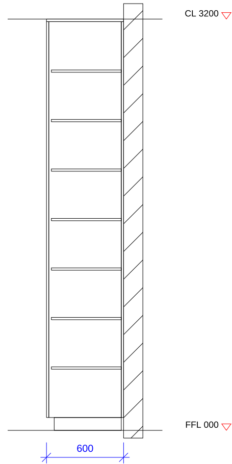
SECTION X-X 1:30
