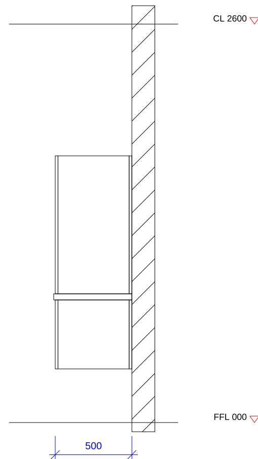
SECTION X-X 1:25
