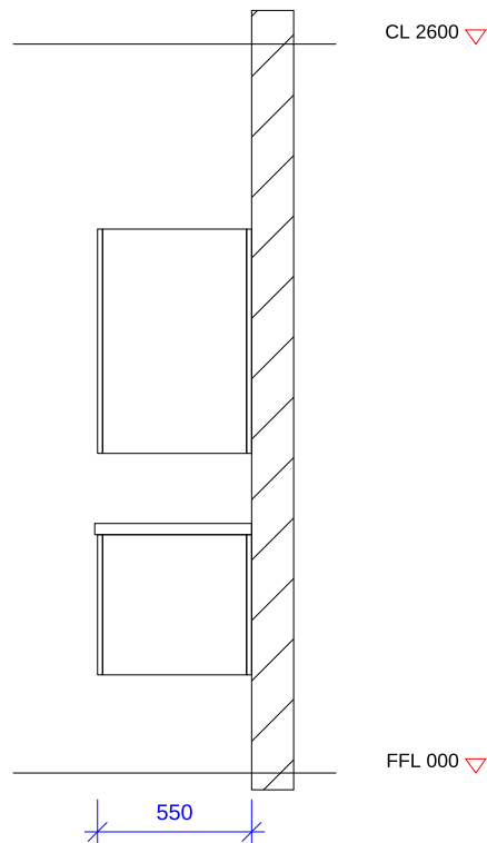
SECTION X-X 1:30
