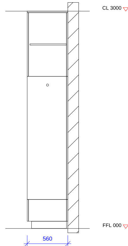
SECTION X-X 1:30
