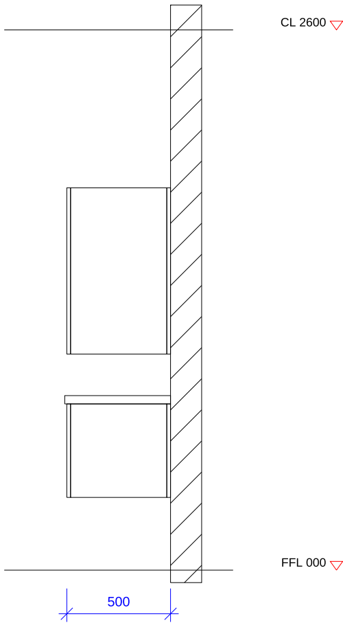
SECTION X-X 1:25
