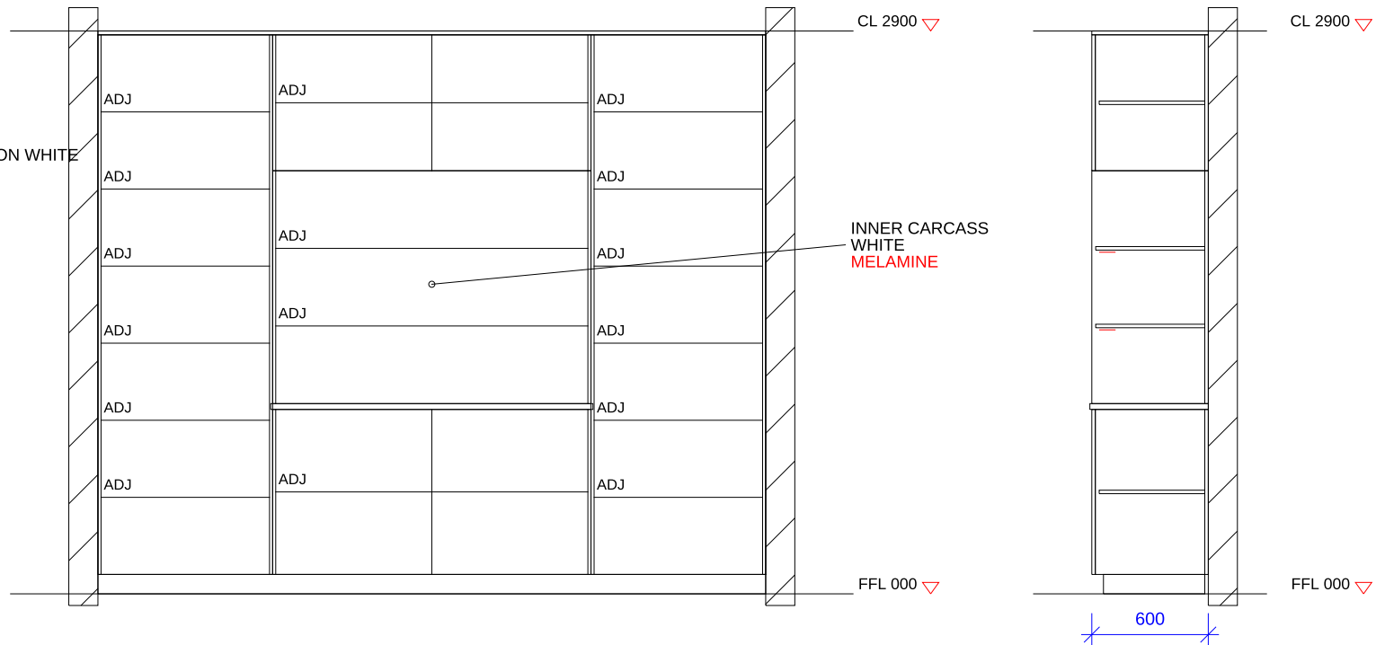
INNER CARCASS A 1:35
