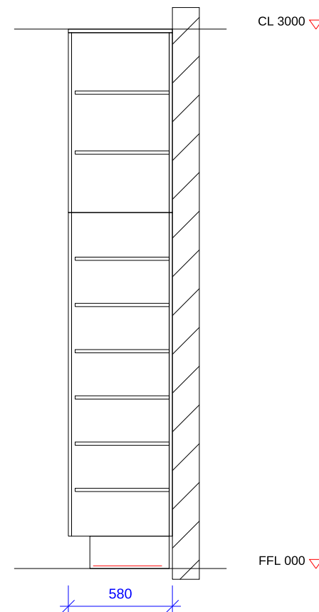
SECTION X-X 1:30
