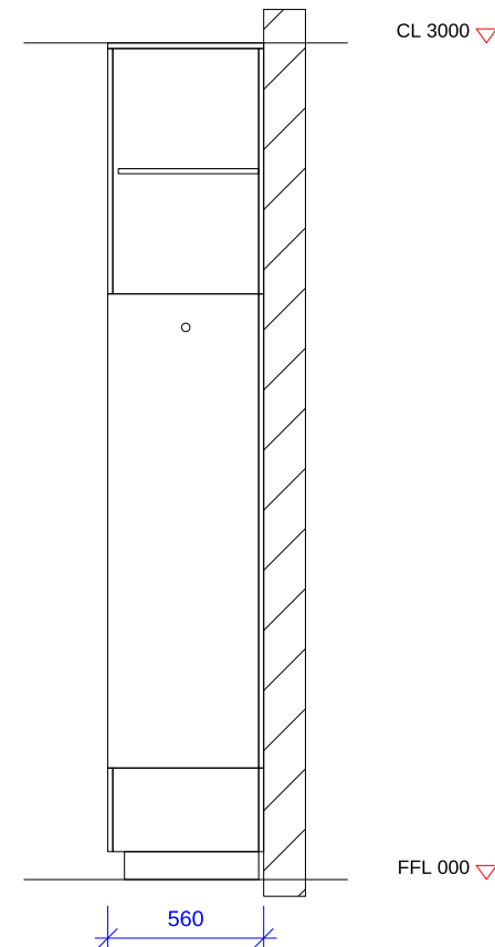
SECTION X-X 1:30
