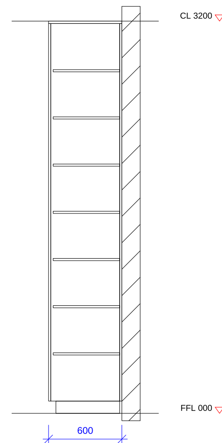
SECTION X-X 1:30
