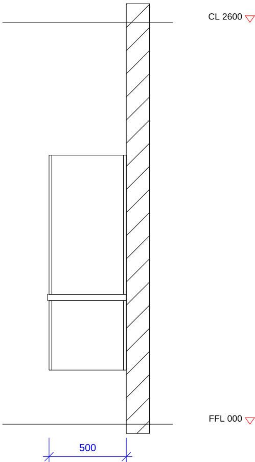
SECTION X-X 1:25
