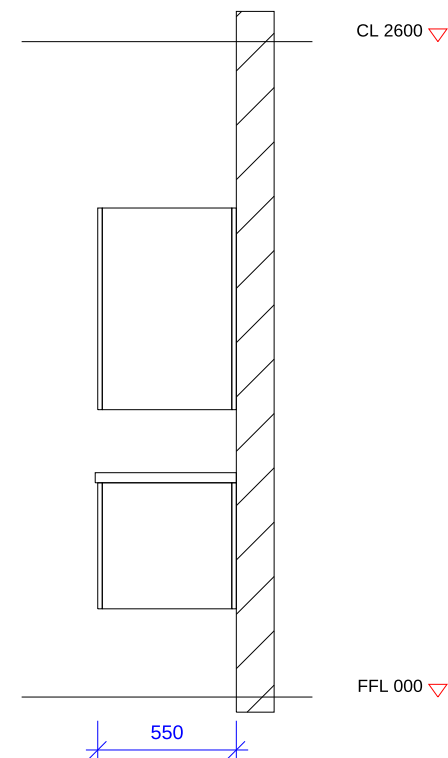
SECTION X-X 1:30
