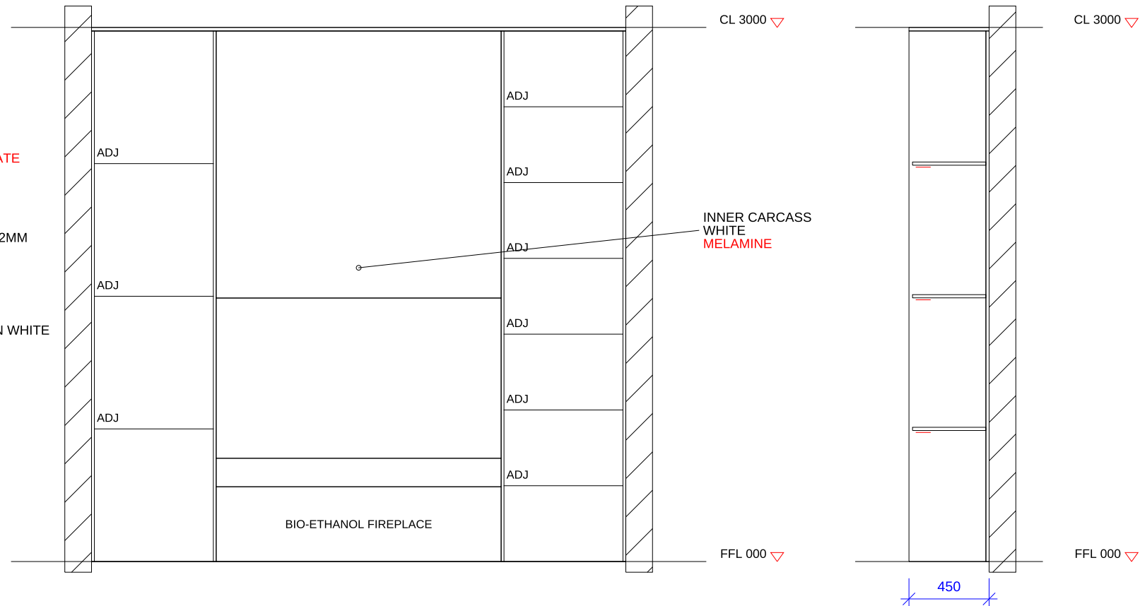
INNER CARCASS A 1:30
