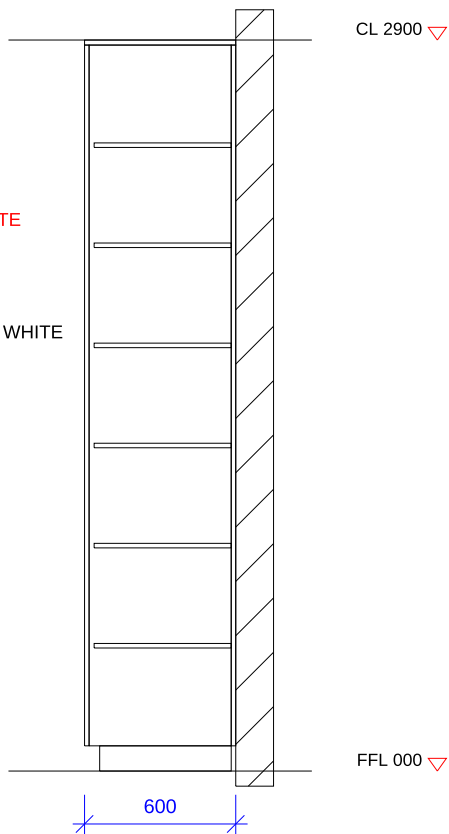
SECTION X-X 1:30
