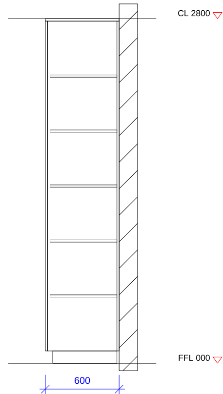
SECTION X-X 1:30
