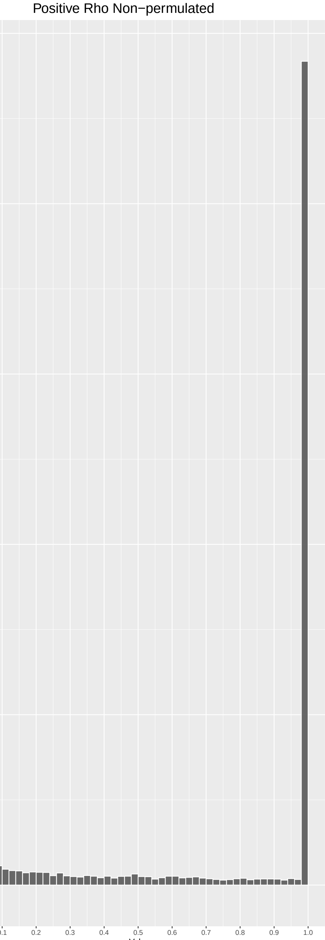
Top Positive genes by P-value non-permulated
