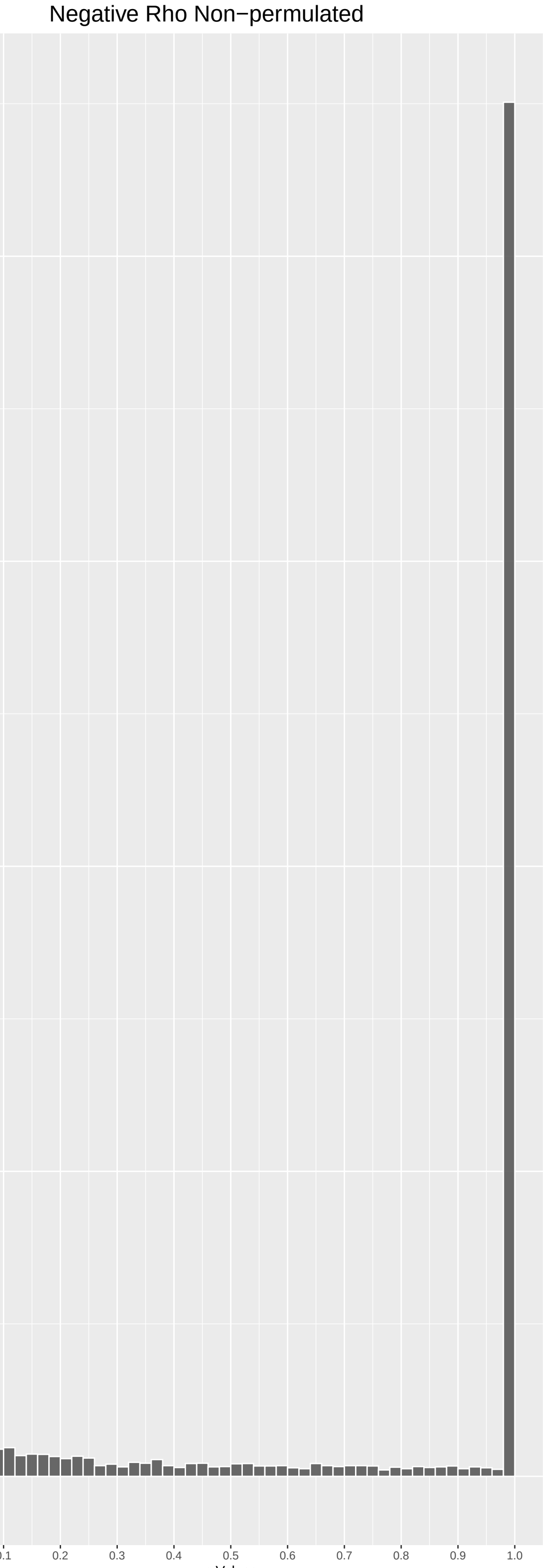
Top Negative genes by P-value non-permulated
