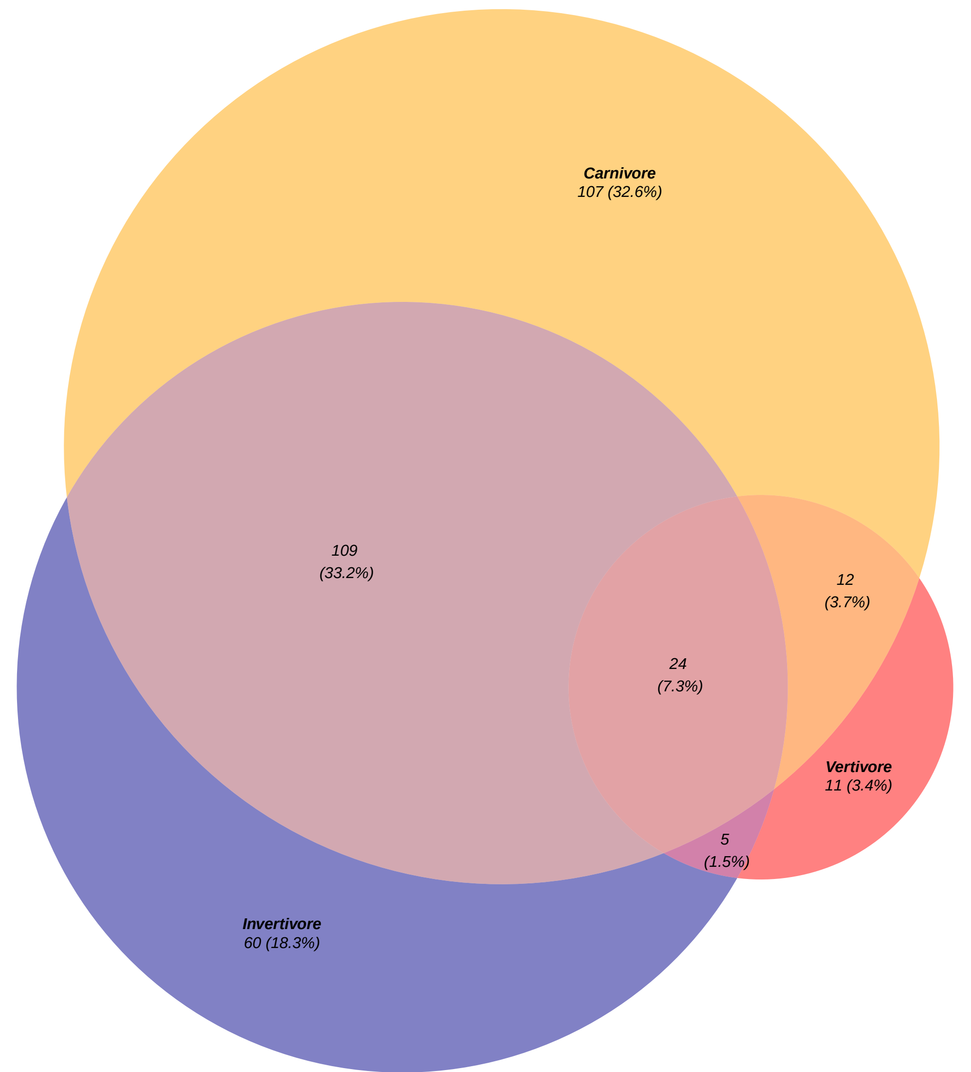
GOCategories (p.adj &lt; 0.05)
