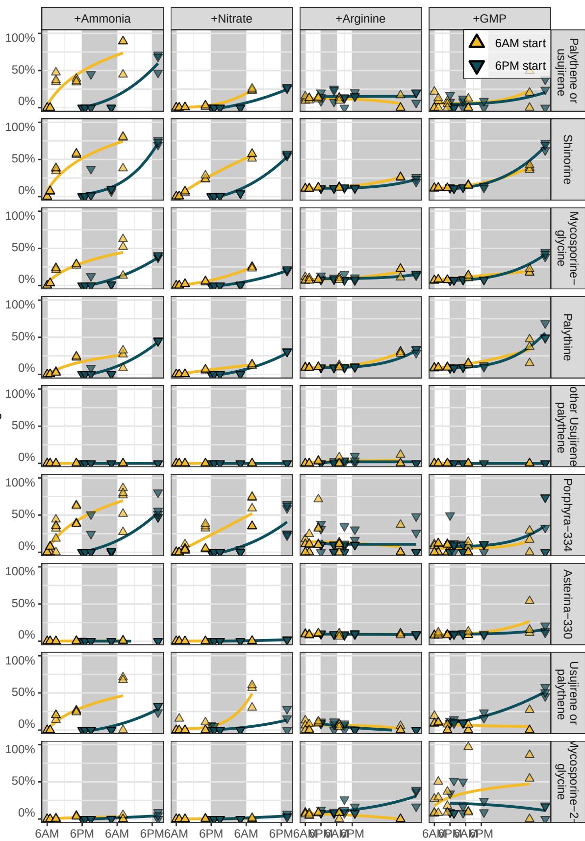
Fraction of MAA containing at least one ^{15}\text{N} atom
