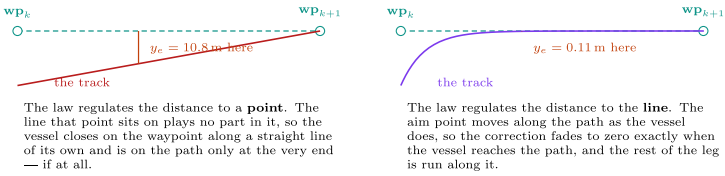
Both vessels start 18 m off the path and both reach the waypoint. Only one travels along the line to it. The tracks are not sketched: the LOS curve is the guidance law integrated along the path, dy_e/ds = -y_e/\sqrt{\Delta^2 + y_e^2} , by _tools/w04.track.curves.awk . Measured on the four-leg mission of section C: atan2 holds the path to 0.547 m and LOS to 0.060 m.
