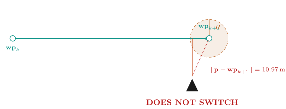
(b) circle of acceptance — what most books draw
