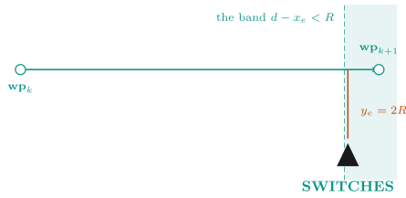
(a) along-track — what MSS uses
