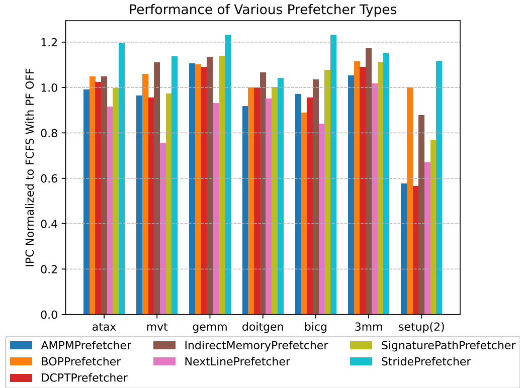
Figure 12 Normalized IPC for various prefetcher types running benchmarks under setup 1 and setup 2
