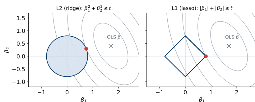
Figure 31: Why lasso zeros coefficients: loss contours meet the L2 disc anywhere, but meet the L1 diamond at a corner.
