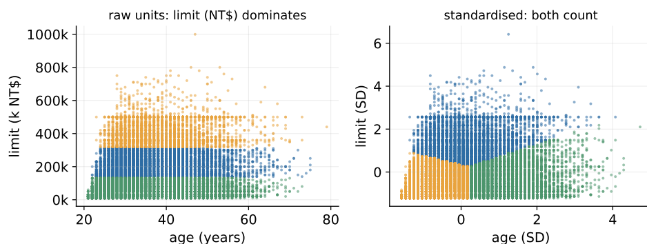
Figure 50: The same two features - credit limit and age - clustered raw and standardised. In raw units, the limit is the only voter.
