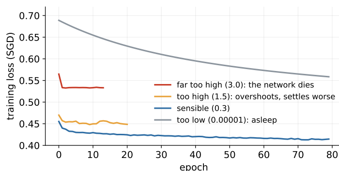
Figure 77: Four learning rates: dead, overshooting, sensible, asleep.
