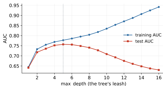
Figure 36: The U-curve, tree edition: max_depth is the leash.
