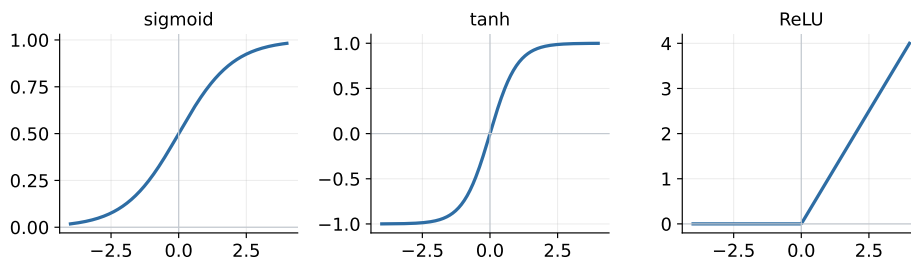
Figure 73: Activations: the bend between the layers.
