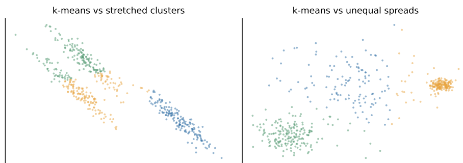
Figure 54: K-means versus shapes that violate its assumptions.
