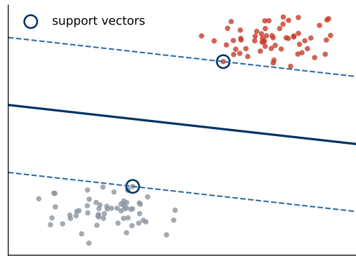
Figure 37: Maximum margin: the boundary rests on the support vectors alone.
