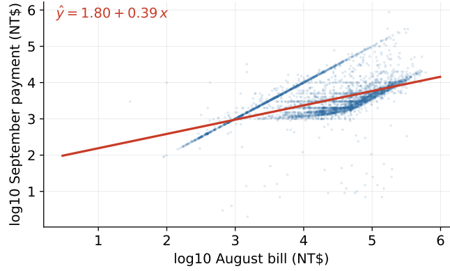
Figure 21: The warm-up fit: log payment on log bill. The slope is an elasticity.
