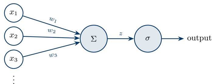
Figure 71: The neuron: the weighted inputs are summed into z , and \sigma squashes z into the output.
