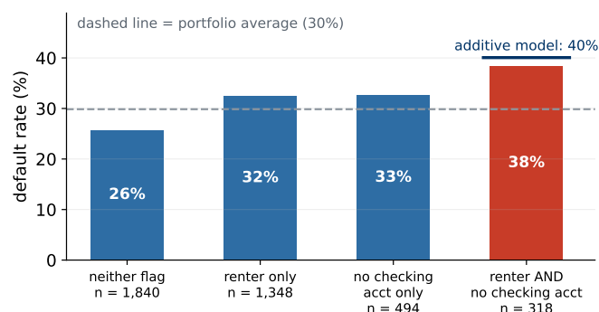
Figure 17: Default rate by the two flags (dashed: portfolio average). Stacking them isolates a riskier segment, but no riskier than an additive log-odds model predicts from the one-flag segments (dark bar).
