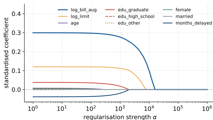
Figure 30: Lasso coefficient paths: features leave the model one by one. Same \alpha axis as Figure 29 (both penalise the sum of squared residuals): the weak features are gone by \alpha \approx 10^3 , where ridge has barely started.
