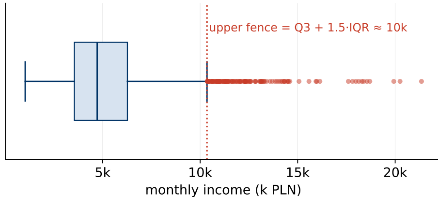
Figure 13: Income with the IQR fence. Every flagged point here is a genuine high earner, not an error.
