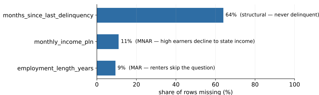
Figure 14: Missingness in the course portfolio: three columns, three mechanisms (known here by construction), three different correct treatments.
