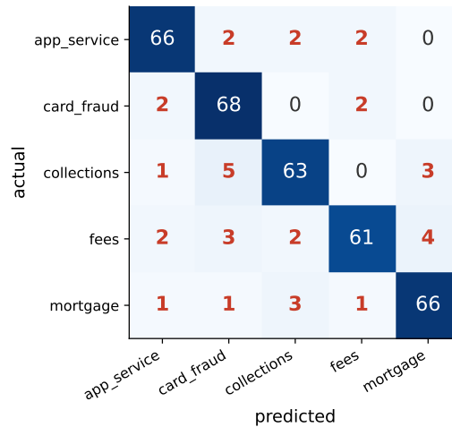
Figure 69: The router's confusion matrix (test set).
