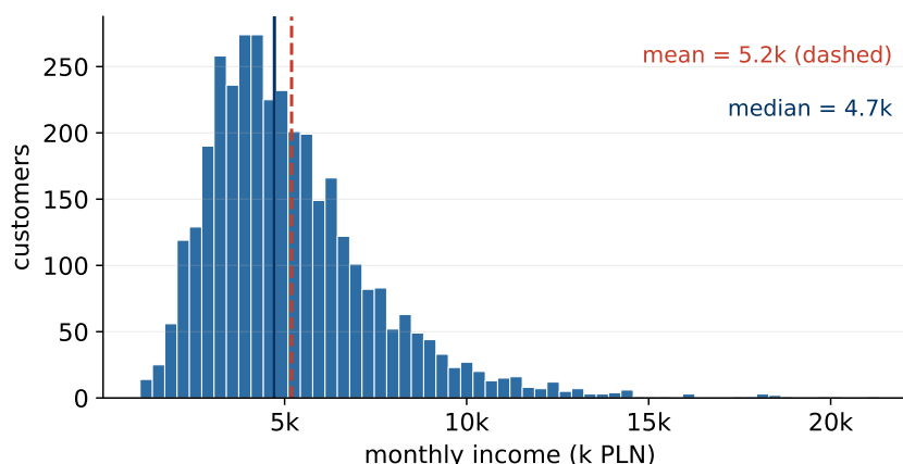
Figure 5: Monthly income: right-skewed, mean above median.
