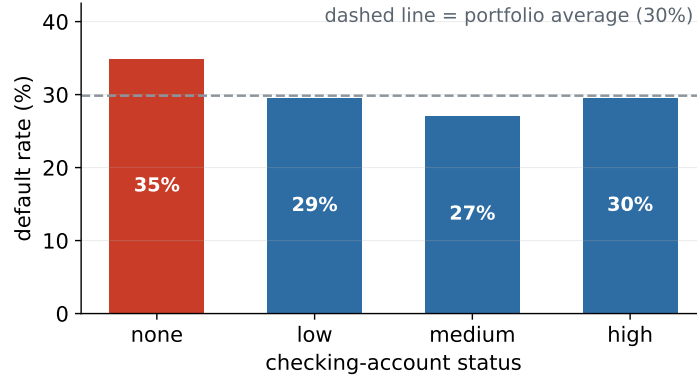
Figure 9: Default rate by checking-account status.
