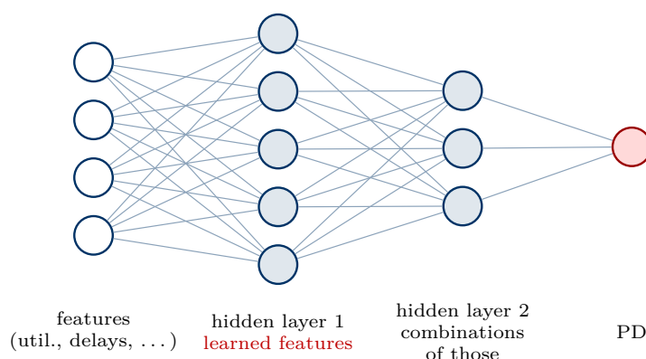
Figure 72: Stack and repeat: the first hidden layer learns features, the second combines them, and the output unit returns the PD (a schematic; the lab network, counted below, is 12 \rightarrow 32 \rightarrow 16 \rightarrow 1 ).
