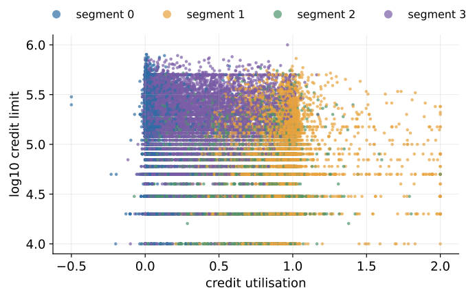
Figure 52: k = 4 on six scaled features, shadowed onto two of them. The wall at zero utilisation is mostly the transactor population.
