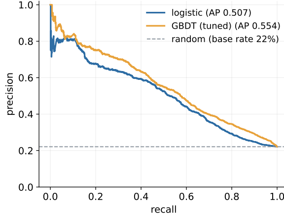
Figure 45: Precision–recall: random guessing floors at the base rate.
