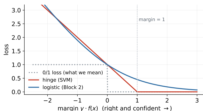
Figure 39: Three losses against the margin yf(x) : 0/1, hinge, logistic.
