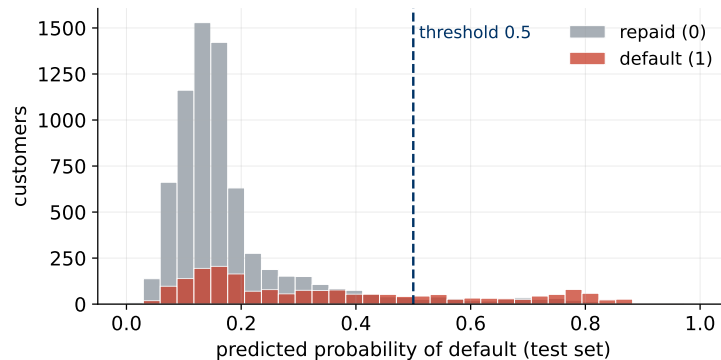
Figure 28: Predicted default probabilities by true class, test set. The overlap is why thresholds are decisions, not constants.
