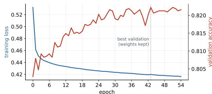
Figure 76: The canonical training plot: validation accuracy plateaus, and early stopping keeps the weights of the best epoch.
