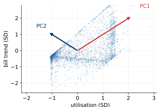
Figure 57: PCA on two correlated features, utilisation and bill trend ( r = 0.56 ): the components are the cloud’s natural axes.
