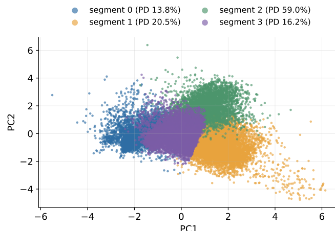
Figure 60: The k = 4 segments in PCA coordinates: transactors and maxed-out borrowers at the two ends of PC1, the distressed apart along PC2.
