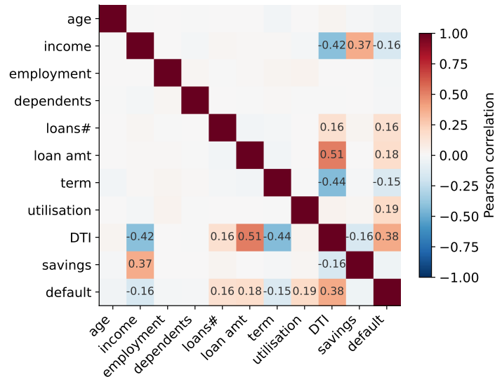
Figure 10: Pearson correlations among numeric features and the target (only |r| \geq 0.13 annotated).
