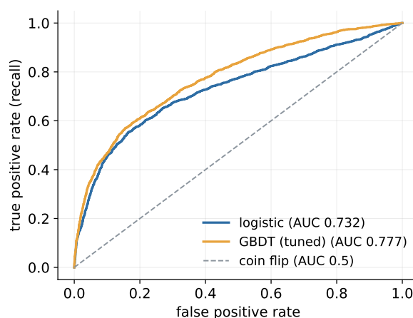
Figure 44: ROC curves for the baseline and the tuned GBDT.
