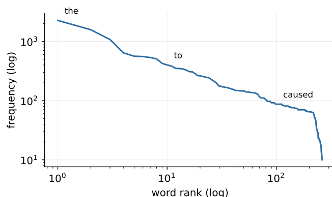
Figure 66: Zipf's law in the complaint corpus.
