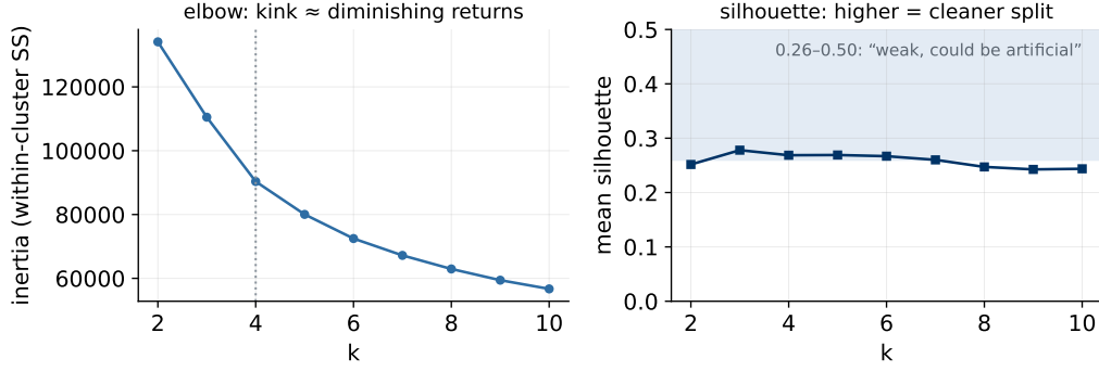
Figure 53: Choosing k : inertia (elbow) and mean silhouette.
