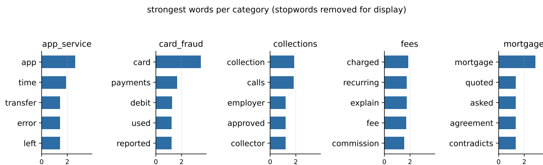
Figure 70: What the model reads: top words per category.
