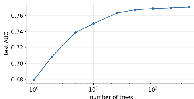
Figure 40: Random forest: more trees plateau, never overfit.
