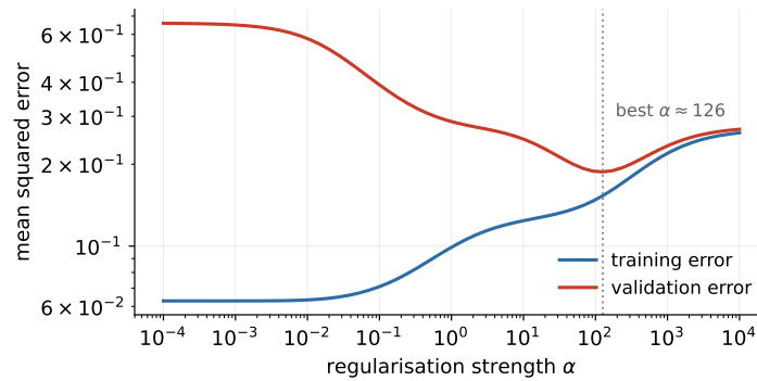
Figure 32: Choosing \alpha : the validation curve on a high-variance setup.
