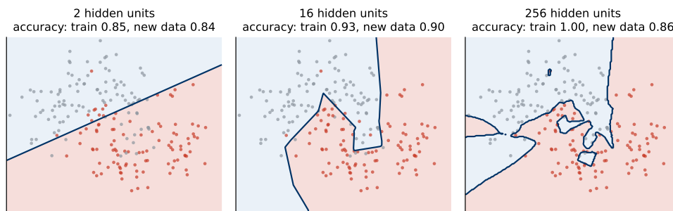
Figure 75: Capacity: width is a dial on the same U-curve (accuracy on the 200 training points and on 20,000 new ones).
