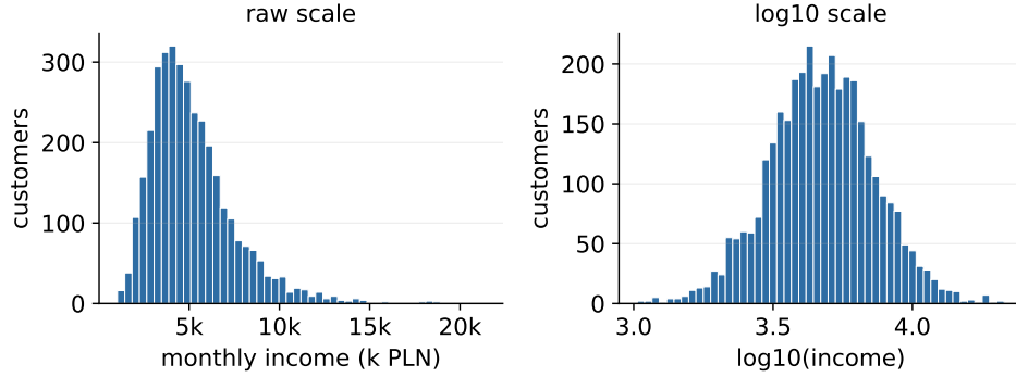
Figure 6: The same income variable, raw and log scale.
