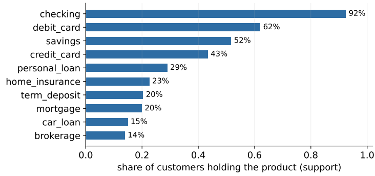
Figure 63: Single-item supports: product penetration.
