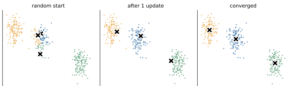
Figure 51: K-means: assign, update, repeat.
