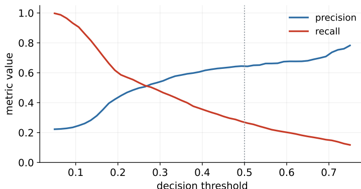
Figure 33: Precision and recall as the decision threshold moves.
