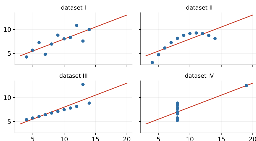
Figure 12: Anscombe’s quartet: identical summaries, different data.
