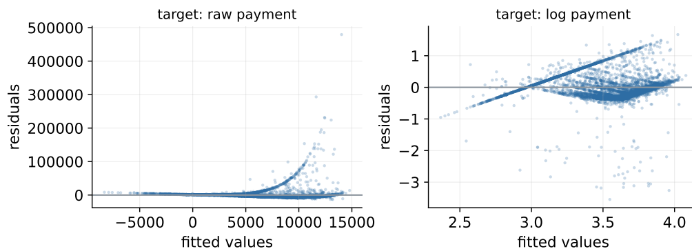
Figure 22: Residuals against fitted values, raw versus log target. The funnel on the left is heteroscedasticity; the log removes it and exposes a mixture - the sharp diagonal stripe is the clients who pay their August bill in full.
