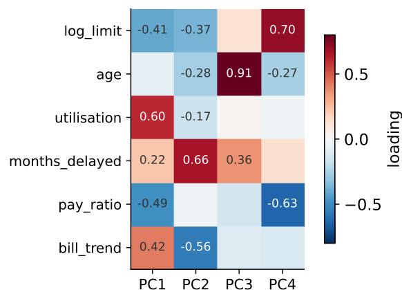
Figure 59: Loadings of the first four components.
