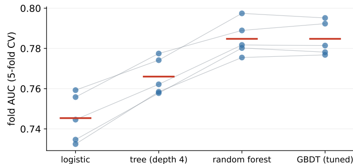
Figure 43: Five-fold CV: fold scores, with a grey line joining each fold across models, and means in red. The first two steps of the ladder hold on every fold; forest and GBDT tie.
