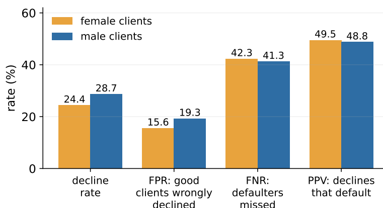
Figure 79: Our own model, audited by sex at the Bayes threshold t = 0.25 .
