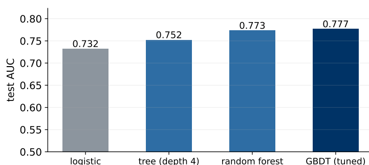
Figure 41: The tournament on held-out data: every rung of the ladder pays.
