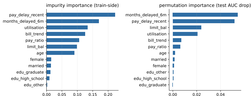
Figure 49: Impurity versus permutation importance for the forest.
