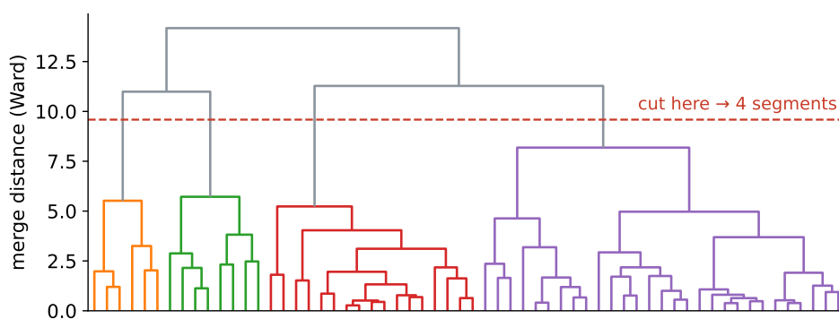
Figure 55: Ward dendrogram on a 60-customer sample, cut to leave four groups.
