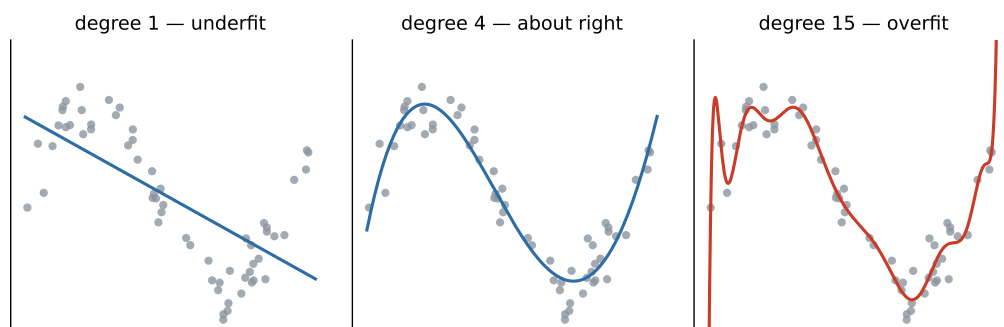
Figure 19: One dataset, three polynomial fits: underfit, about right, overfit. The overfit curve fits the training points best - exactly why training error cannot be trusted.
