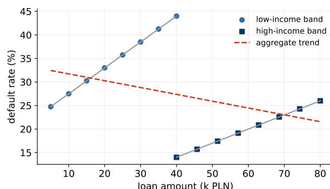
Figure 11: Simpson’s paradox (illustrative data): the aggregate slope (dashed) reverses the within-group slopes.
