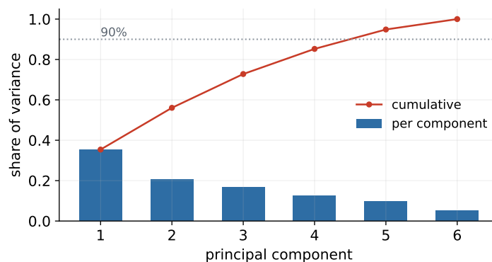
Figure 58: Scree plot: some redundancy, moderate compression.
