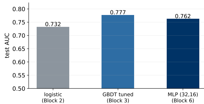
Figure 78: The final tournament: the MLP beats the baseline, not the GBDT.
