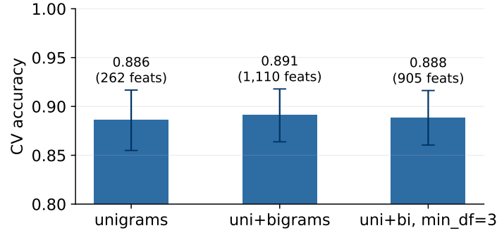
Figure 68: N-grams cost dimensions; here they buy half a point, inside the fold-to-fold spread (error bars).
