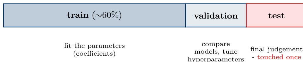
Figure 18: A typical three-way split, one job per sample: the training sample fits the coefficients, the validation sample chooses between models and settings, and the test sample gives the final verdict - once.
