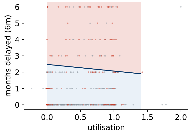
logistic: one straight cut
