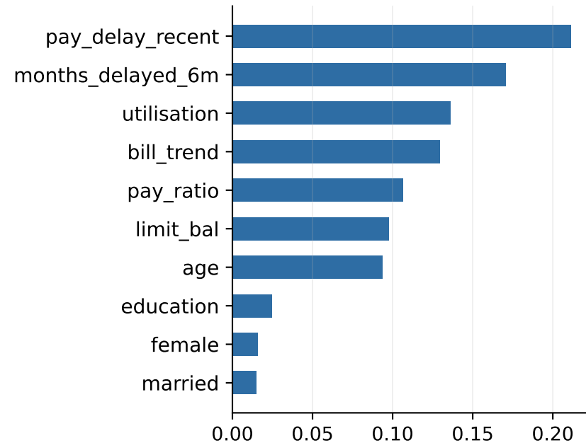
impurity importance (train-side)
