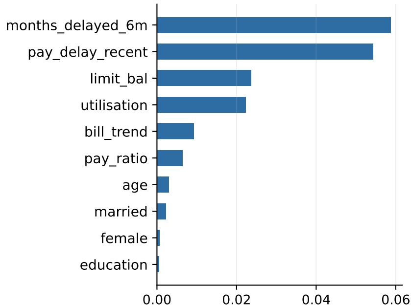
permutation importance (test AUC drop)
