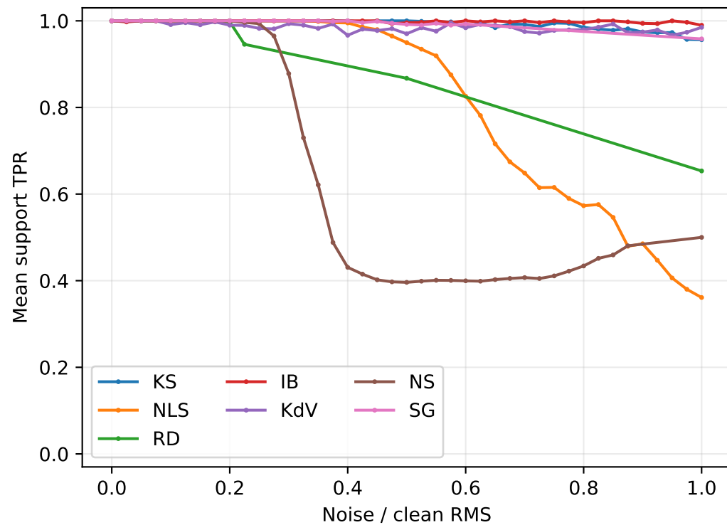
WSINDy authors — partial results; n=20-200 per noise level
