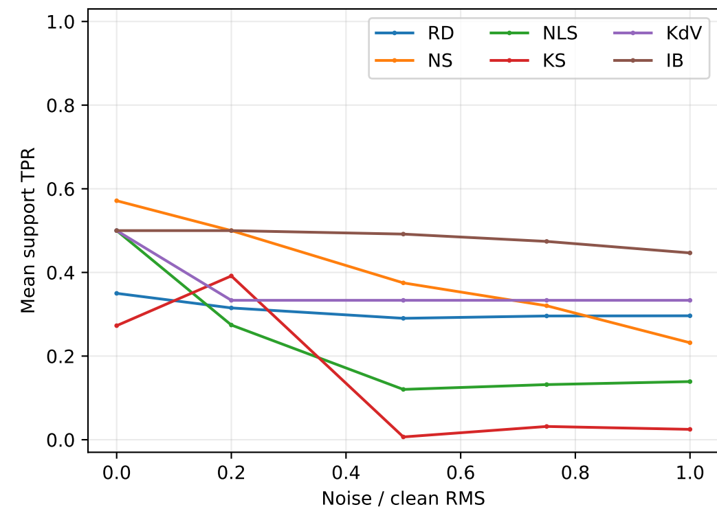
Filtered WSINDy + LASSO authors — complete; n=100 per noise level
