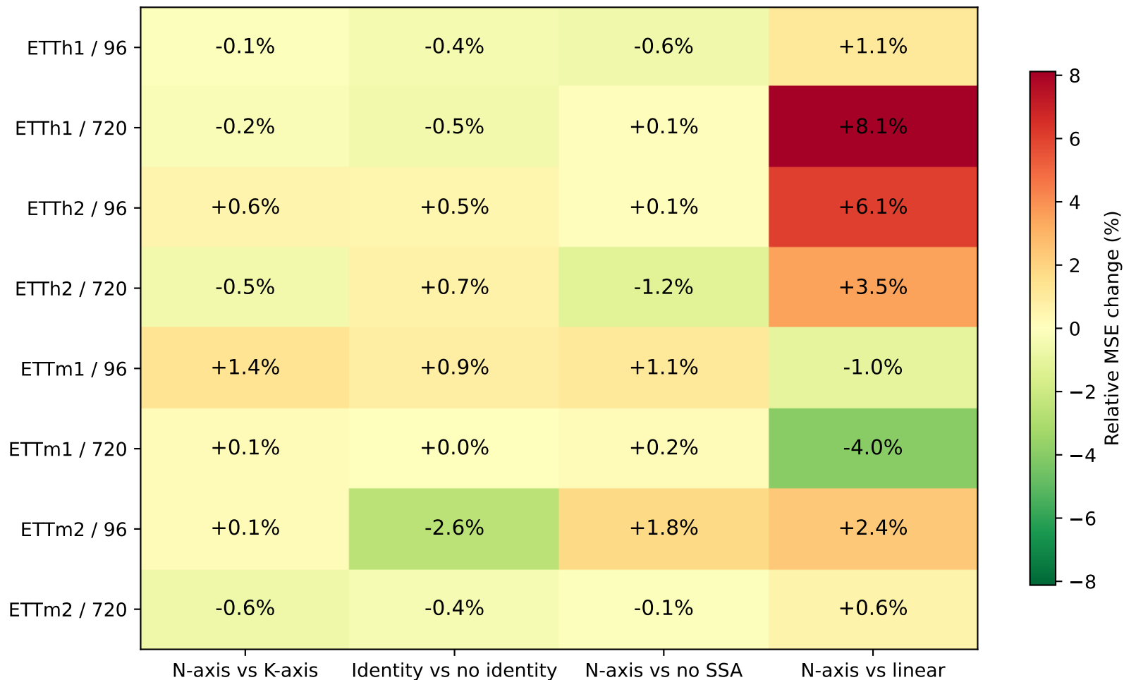
Relative test MSE: negative means improvement
