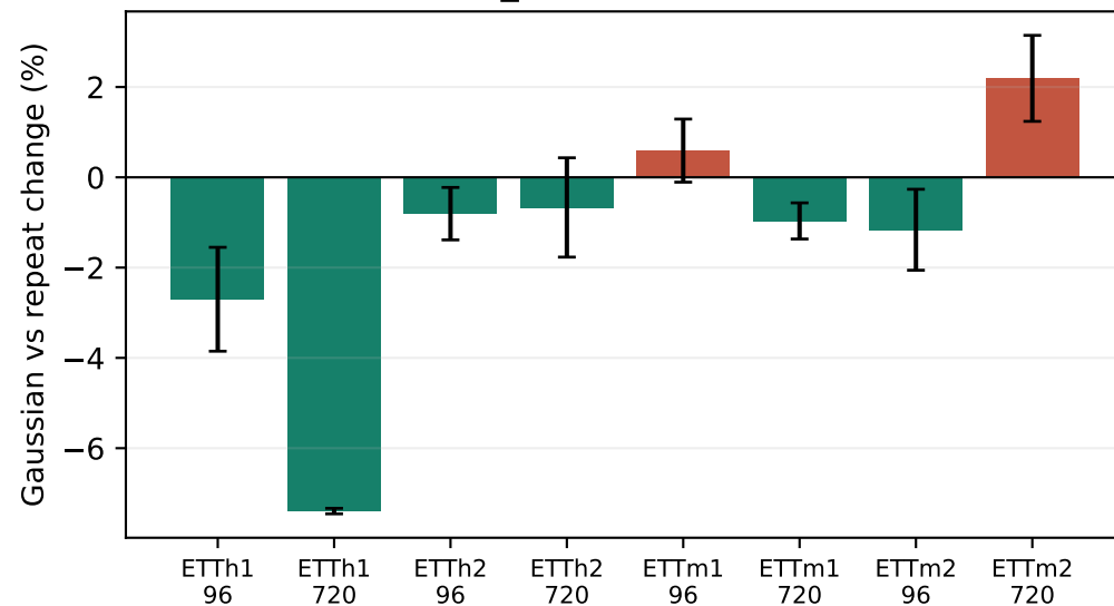
no_attention / MAE
