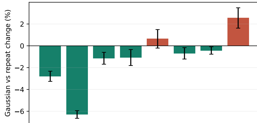
temporal / MAE
