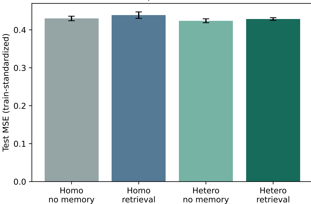
Causal population Spike-TCN: mean \pm sample SD over 3 seeds
