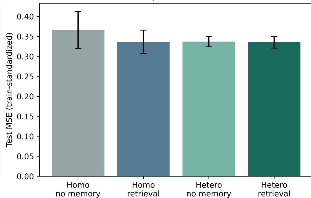
Causal population Spike-TCN: mean \pm sample SD over 3 seeds
