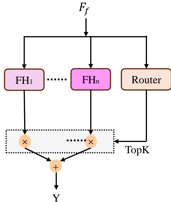
Unified Feature Harmonizer (UFH)
