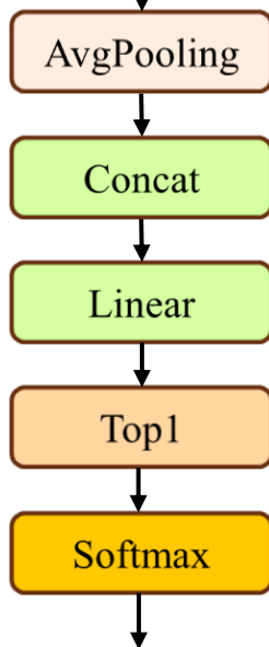
Router [F_R, F_T]
