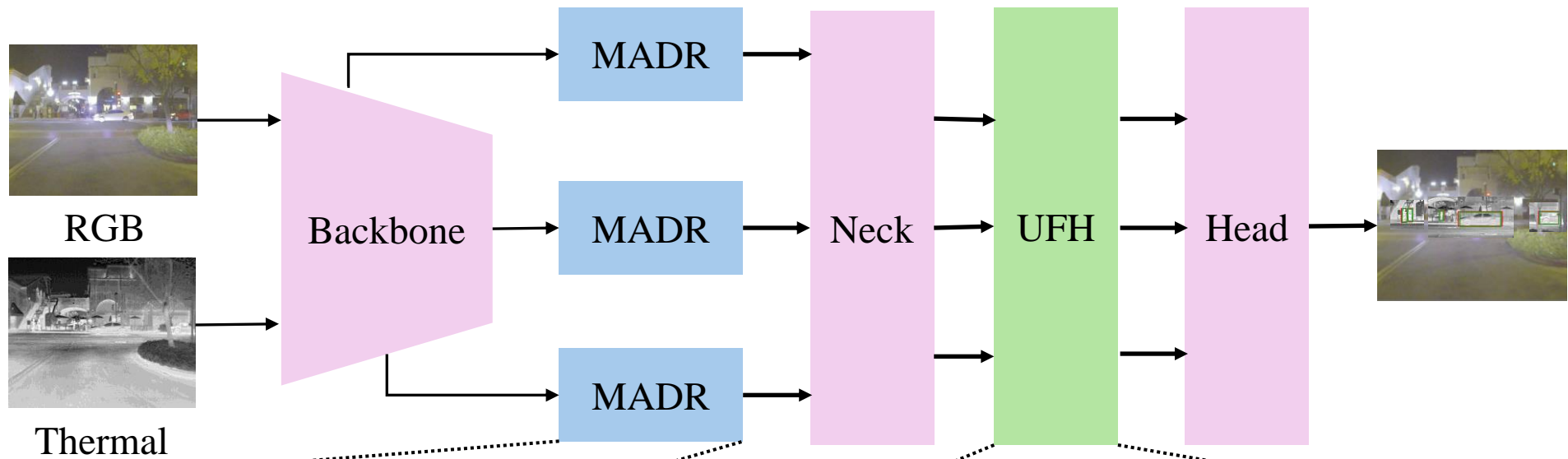
Modality-Aware Dynamic Routing (MADR)
