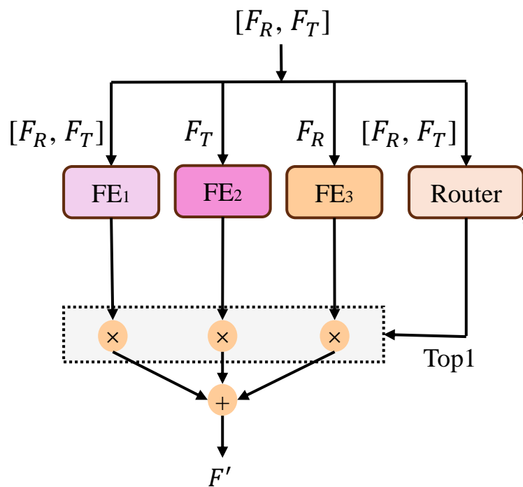
Modality-Aware Dynamic Routing (MADR)
