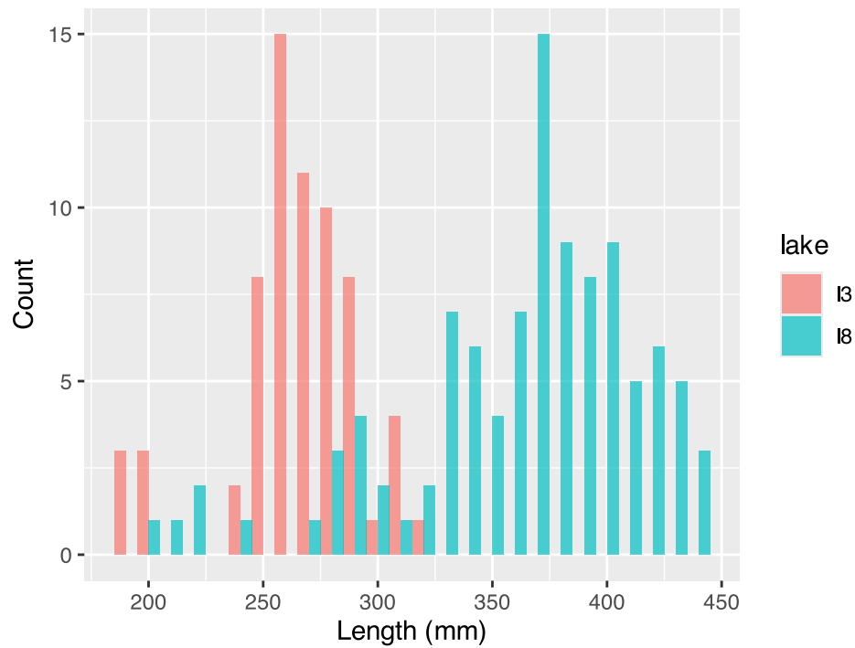
Arctic grayling length data from lakes I3 and I8
