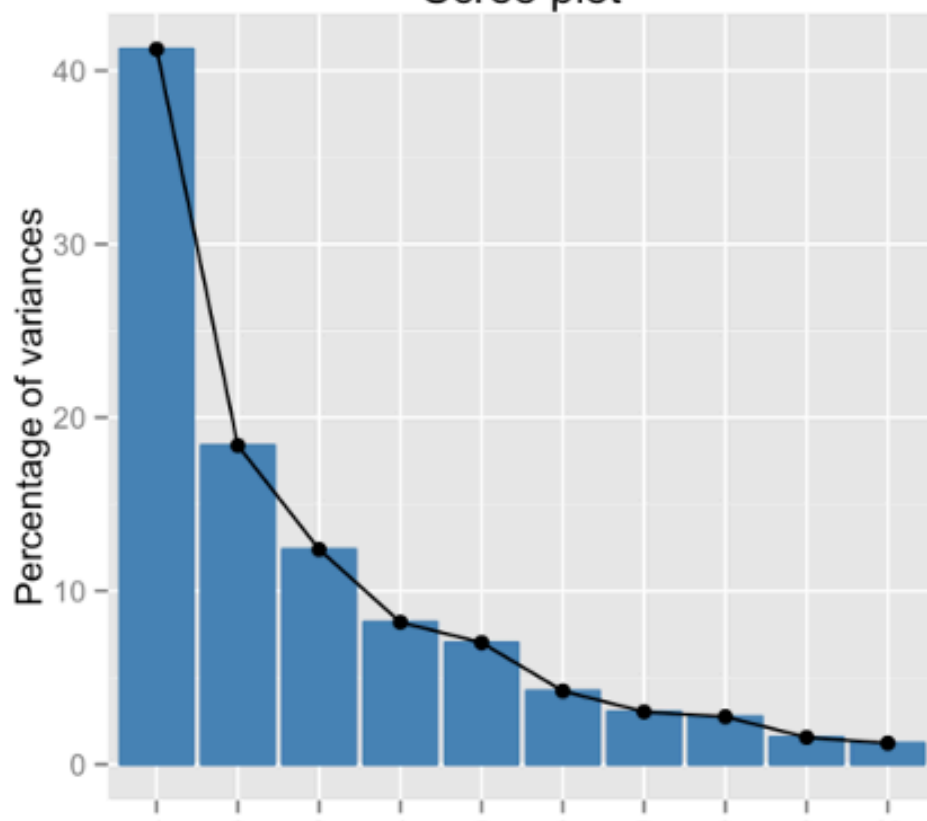
Scree plot
