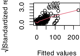
Scale-Location
