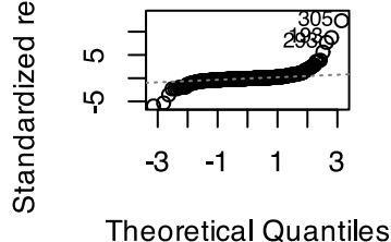
Q-Q Residuals
