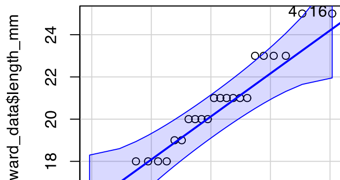
QQ Plot: Leeward Needles
