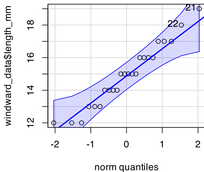
QQ Plot: Windward Needles
