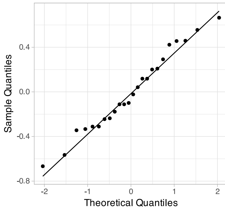
Q-Q Plot of Residuals
