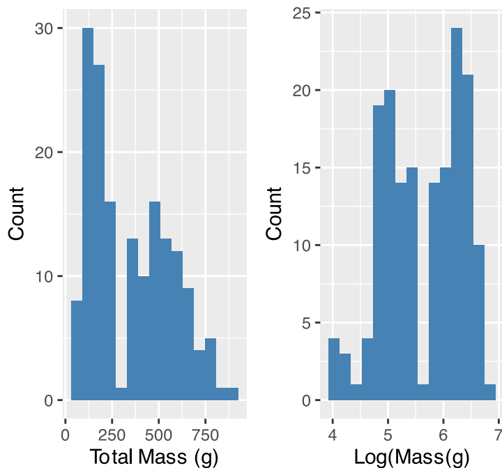
Original Mass Distribution Log-Transformed Mass Distribution
