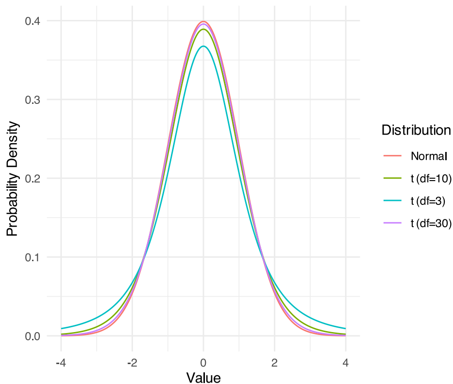
Comparison of Normal and t-distributions
