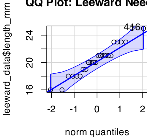
QQ Plot: Leeward Needles
