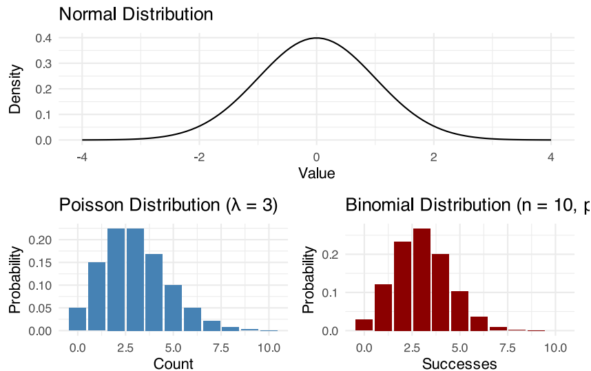
Figure 1: Examples of distributions in the exponential family
