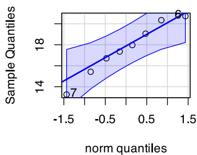
QQ Plot for shady needle leng
