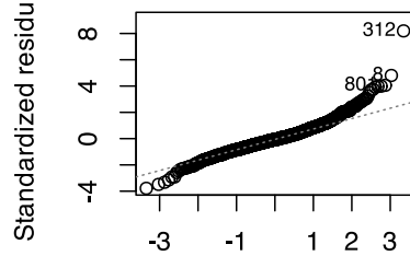
Q-Q Residuals
