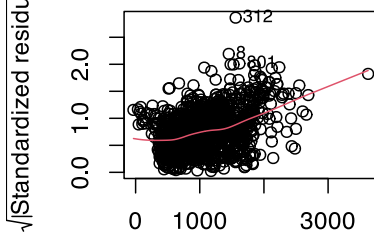
Scale-Location
