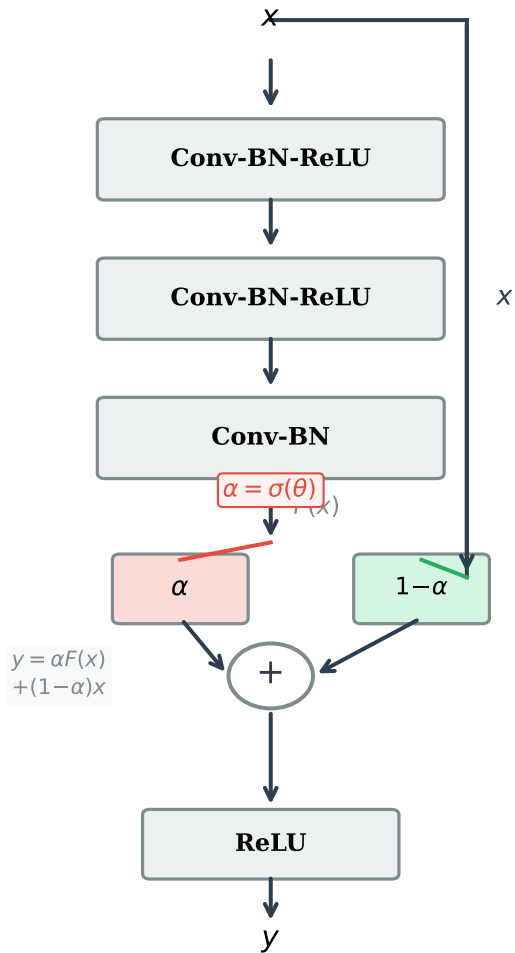
(b) LRS Block (Proposed)
