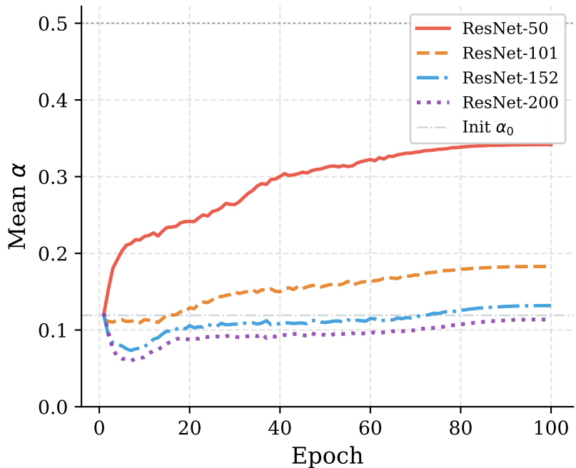
(b) LRS-Low: CIFAR-100
