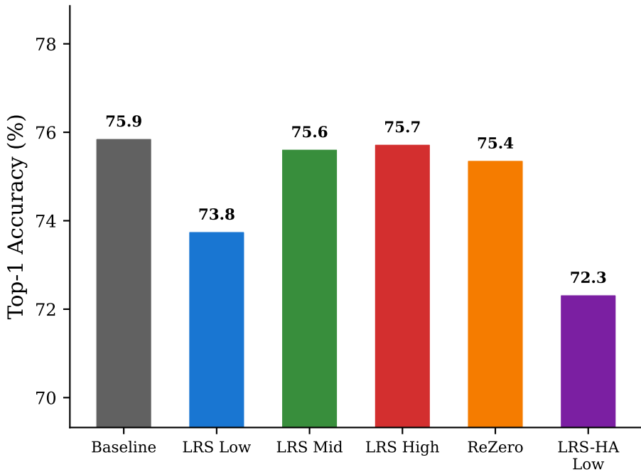
(a) ImageNet Top-1 Accuracy
