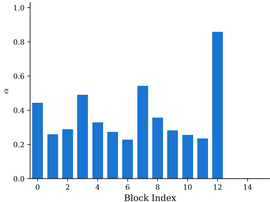
(b) Per-block \alpha (LRS Low, ImageNet)
