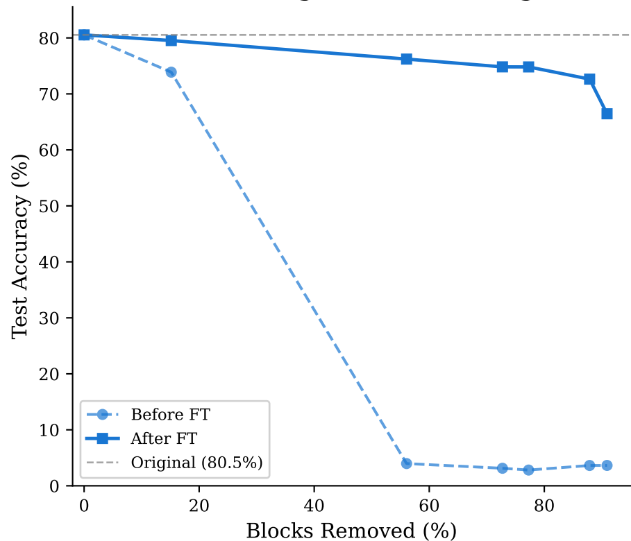
(b) Pruning With Fine-tuning
