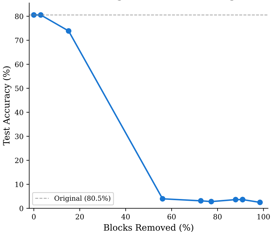
(a) Pruning Without Fine-tuning
