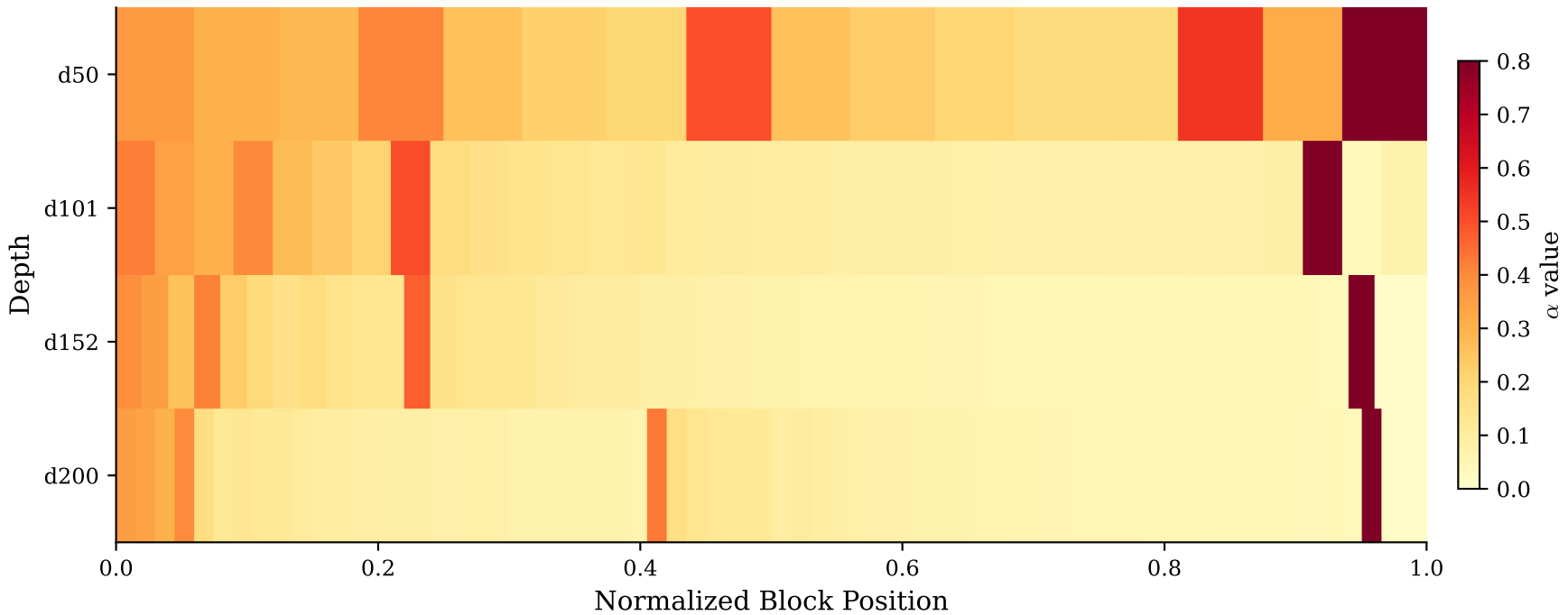
Per-block \alpha Heatmap (LRS Low, CIFAR-100)
